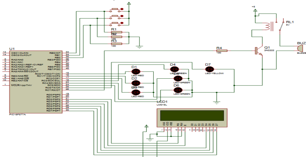
Figure 3: Control circuit.
