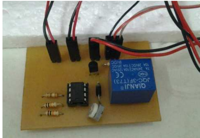
Figure 4: Sensor circuit.
