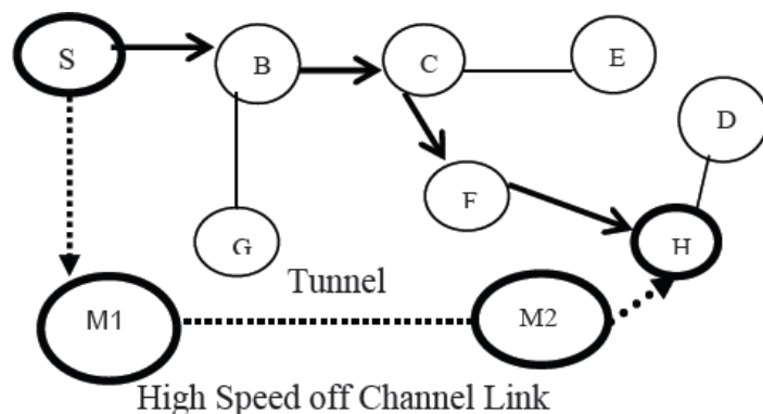
Figure 1: The wormhole attack in MANET
