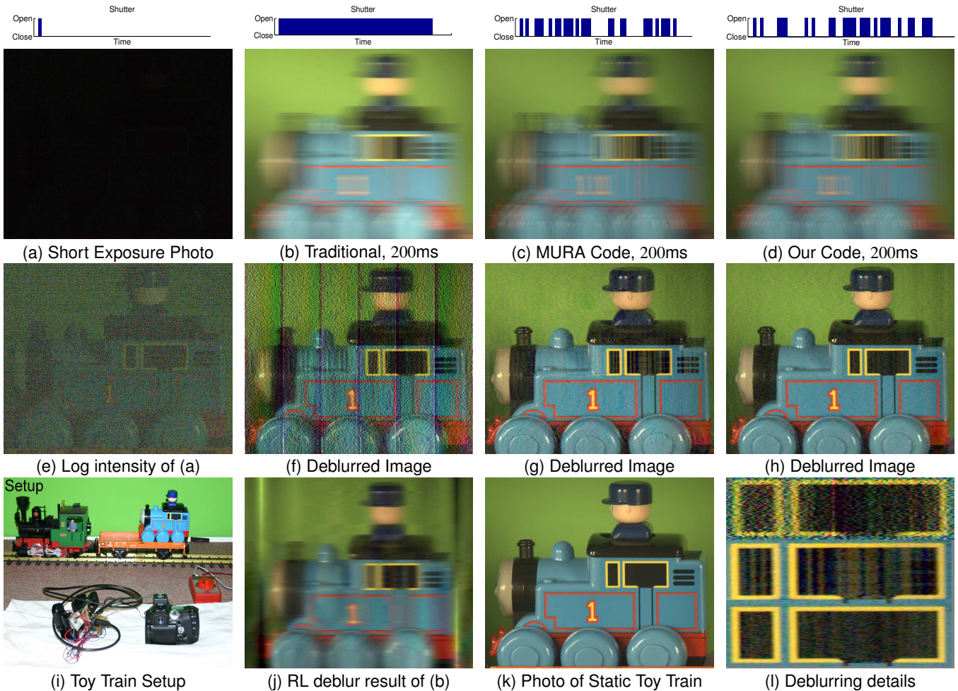
Figure 6: Comparison with other exposure settings: short exposure, traditional shutter exposure, MURA code and our code. The blur in each case is between 118 and 121 pixels, which is 16% of the length of the toy. (a,b,c,d) Shutter sequence and corresponding photos used as input images. (e) Log intensity for short exposure. (f,g,h) Deblurred results using a linear solution. (i) Experimental setup with toy train. (j) Flat blurred image deblurred using Richardson-Lucy (RL) algorithm. (k) Photo of static toy train. (l) Enlarged regions taken from deblurred results for flat (top), MURA (middle) and coded exposure (bottom). Datasets and source code available at http://www.merl.com/people/raskar/deblur/ .
