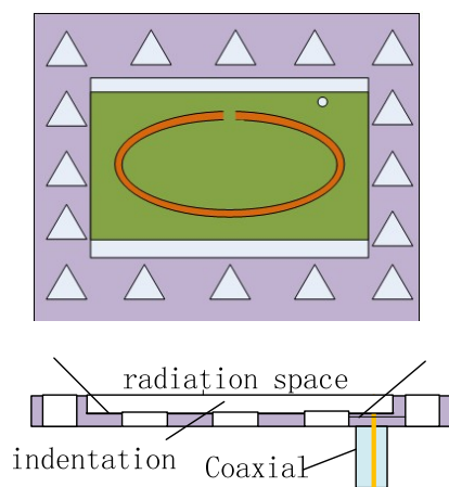
Fig. 4. PBG antenna top view and front view.
