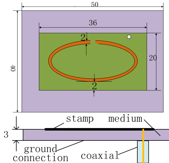
Fig. 1. Top view and side view of the antenna.
