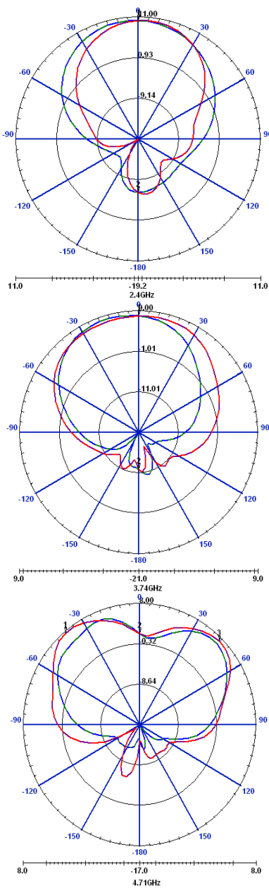
Fig. 3. C-type slot antenna radiation patterns microstrip.
