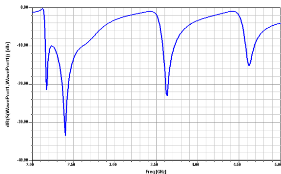
Fig. 5. PBG structure of the antenna return loss graph.
