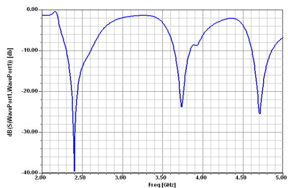
Fig. 2. C-type slot microstrip antenna return loss graph.
