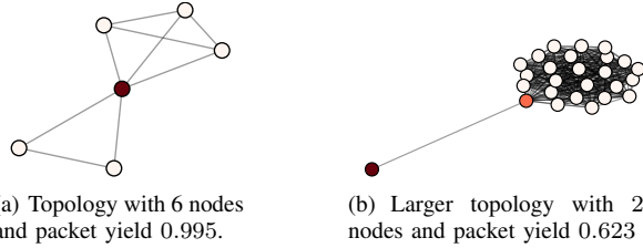
Figure 10. Topologies for CTP exploration on the Pareto front. Darker node color indicates proximity to the gateway node, i.e., the darkest node is the gateway. Note that nodes are arranged to show connectivity, rather than the physical location determined by the MOEA.
