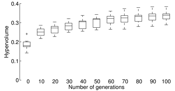
(b) Hypervolume of the MOEA generations (in steps of 10). Boxplots of 10 runs.
