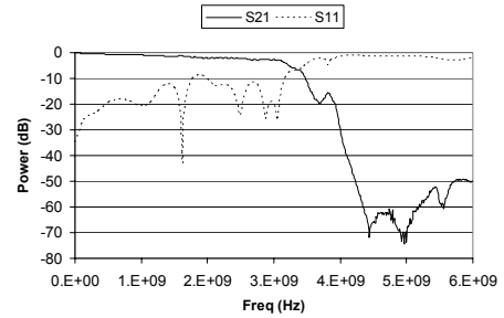
Fig. 5. Measured S21 and S11 of 3GHz LPF.
