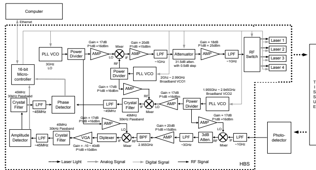
Fig. 1. Block diagram of the HBS.
