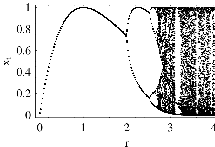
Figure 3.8: Bifurcation diagram of the ricker model (3.8).
