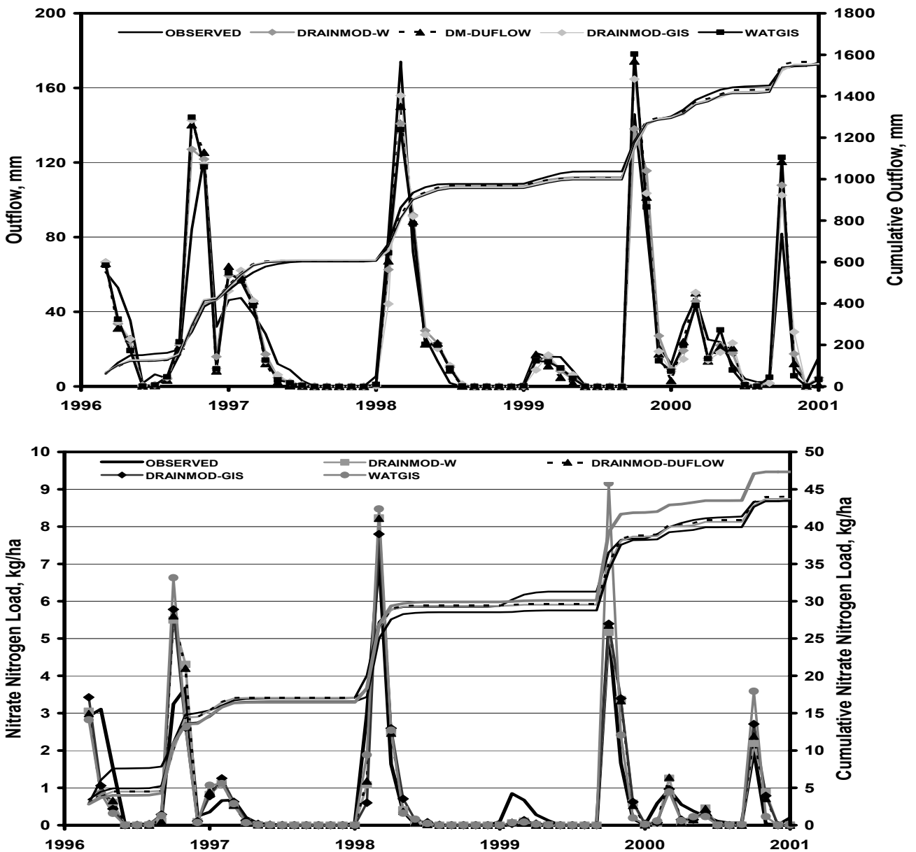
Figure 3. Predicted and measured outflows (top) and nitrate nitrogen loads (bottom) for the forested watershed, S4.
