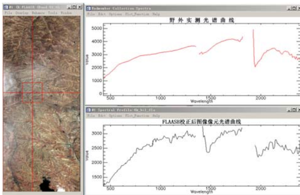
Figure 5 Contrast of Field Measured Spectral Curve and Pixel Spectral Curve
