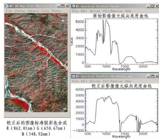
Figure 2 effect image of ELC (vegetation pixel)
