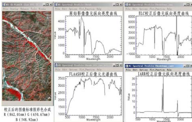
Figure 4 Contrast of Three Correction Methods (uncovered rock pixel)
