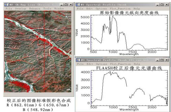
Figure 3 Effect Image by FLAASH (Vegetation Pixel)
