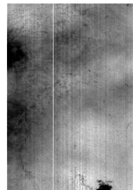
Figure 6 Vapor Water Image Produced by FLAASH with the Fourth Scene of Data
