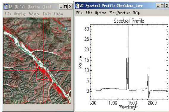
Figure 1 Effect Image by IARR (Vegetation Pixel)
