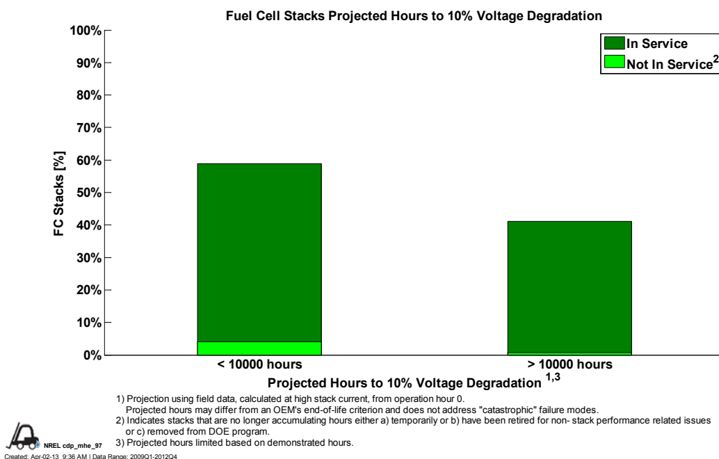
FIGURE 3. Study of Fuel Cell MHE Voltage Degradation Against an Interim Metric Of 10,000 Hours
