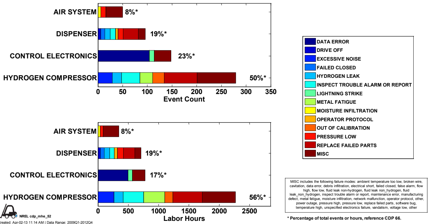
FIGURE 4. Breakdown of Failure Modes for the Top Four MHE Infrastructure Maintenance Categories
