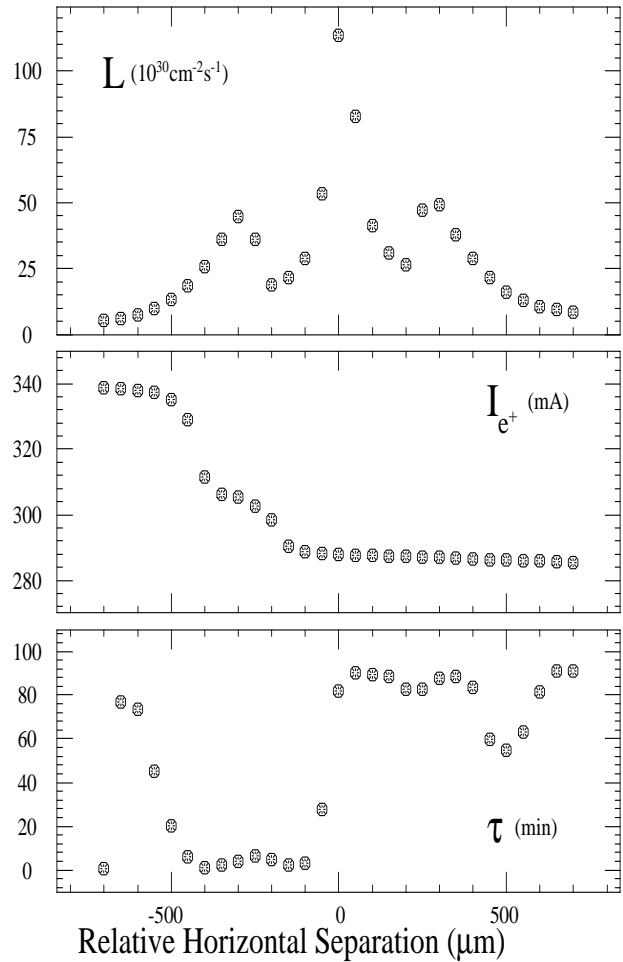
Figure 4: Measured luminosity (top), positron current (middle), and positron beam lifetime (bottom) during a horizontal beam-beam scan with 522 colliding bunches. The total electron current was 200 \text{ mA} .
