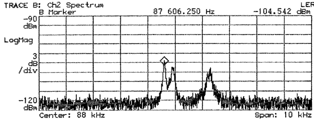
Figure 5: Measured coherent dipole modes. The peaks from left to right are the unperturbed positron vertical tune (measured before injecting electrons), the \sigma -mode, and the \pi -mode.
