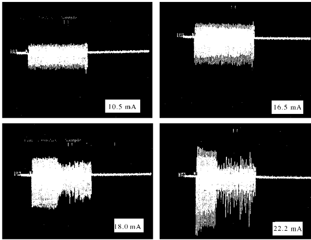
Figure 7: Bunch intensity monitor data with a 100-bunch train with the nominal bunch spacing and transverse multi-bunch feedback turned off.
