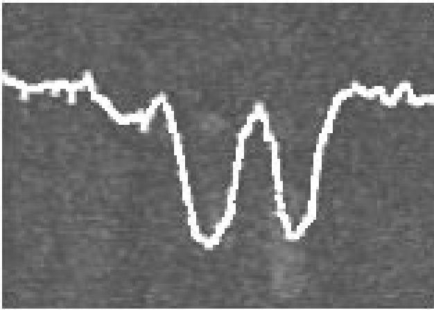
Figure 3: Measured positron beam current during a horizontal beam-beam scan with 1 colliding bunch. The electron current was constant at 0.2 \text{ mA} . The full scales on the horizontal and vertical axes respectively are 8 minutes and 0.5 \text{ mA} .
