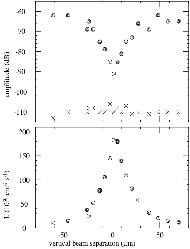
Figure 11: Measured horizontal (crosses) and vertical (circles) instability amplitude (top), and luminosity (bottom) versus relative separation of the colliding electron and positron beams. In this measurement the total currents of the 786 colliding electron and positron beams was respectively 315 mA and 450 mA.
