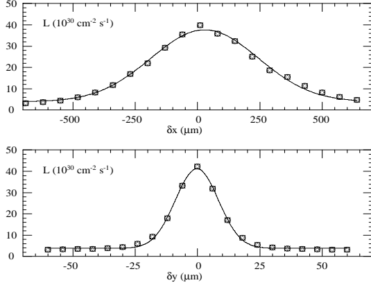
Figure 2: Measured luminosity as a function of horizontal (top) and vertical (bottom) beam separation at the IP with N_c = 786 , I_{e^+}^{\text{tot}} = 280 \text{ mA} , and I_{e^-}^{\text{tot}} = 60 \text{ mA} .
