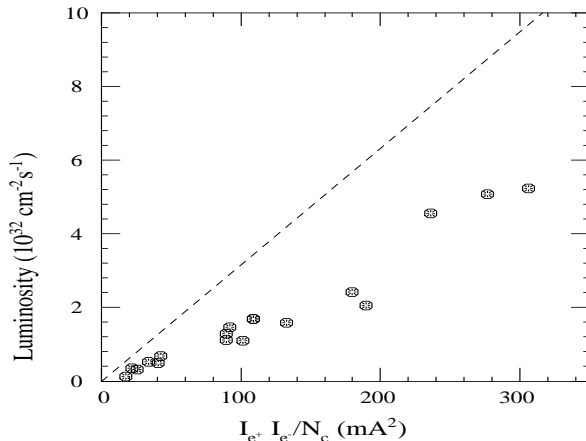
Figure 12: Measured luminosity as a function of the product of the beam currents scaled by the number of colliding bunches. These data were taken with 786 bunches and positron/electron currents in the range of 275-720/60-350 mA respectively. The dashed line shows the expectation assuming design parameters.
