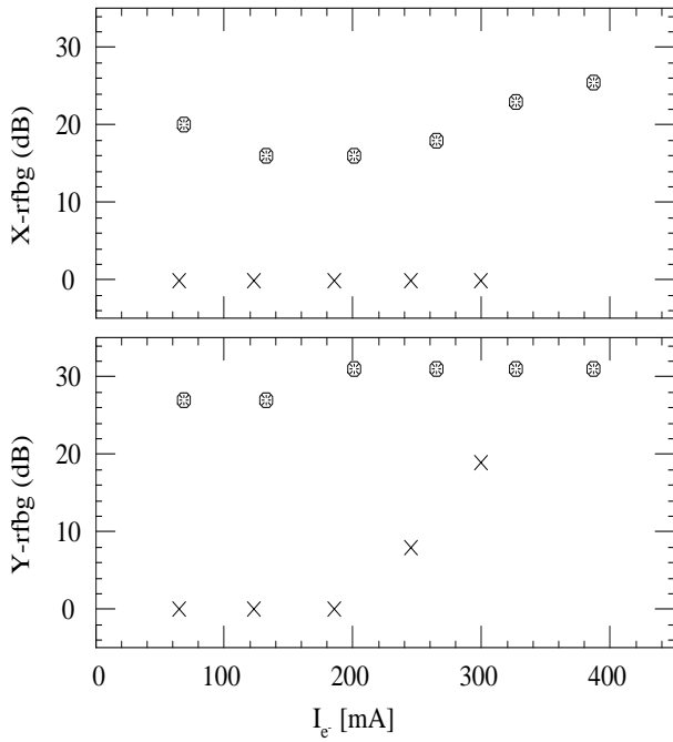
Figure 10: Required feedback gain (rfbg) versus electron beam current with beams in (crosses) and out (circles) of collision in the horizontal (top) and vertical (bottom) planes. In this measurement the total positron beam current was fixed at 0.5 A and there were 786 colliding bunches.
