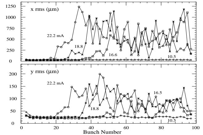
Figure 9: Growth in distribution of horizontal (top) and vertical (bottom) bunch centroid motion along a 100-bunch train with bunches spaced by two buckets.
