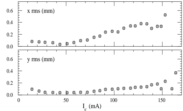
Figure 6: Threshold measurement in the electron ring with transverse feedback off in the horizontal (top) and vertical (bottom) planes.
