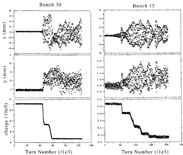
Figure 8: Transverse motion of selected bunches in a 50 bunch train recorded as transverse feedback was turned off. Plotted are the measured horizontal (top) and vertical (middle) beam centroid positions, and the beam intensity (bottom) measured in the HER.
