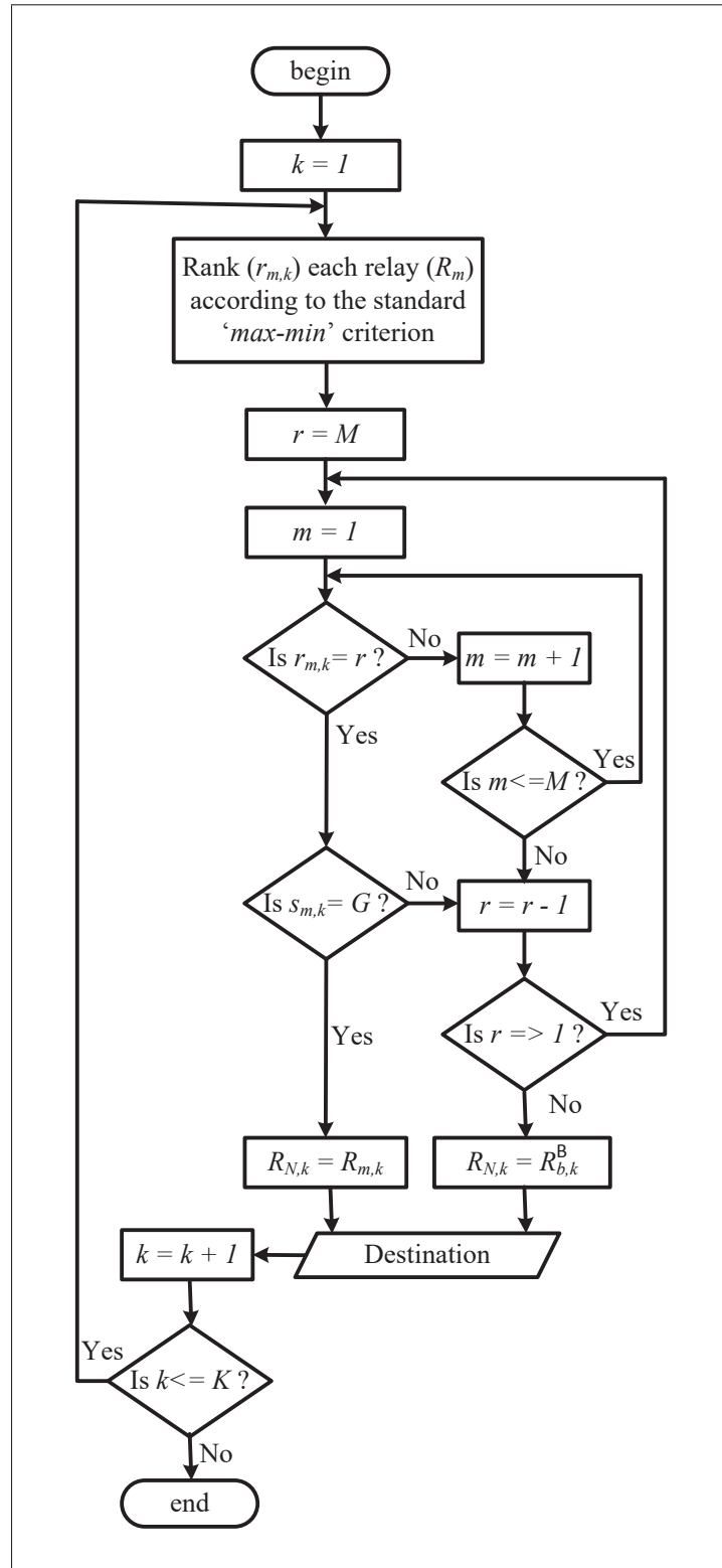
Figure 4.2 Flow diagram of the proposed N 'th BRS protocol in the presence of bursty impulsive noise
