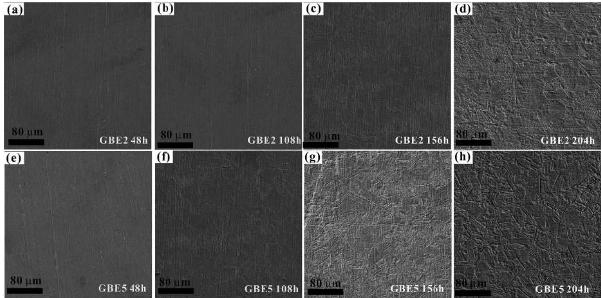
Fig. 14. Morphological maps of GBE2 and GBE5 samples after corrosion in a neutral environment for different times: (a–d) GBE2; (e–g) GBE5.
