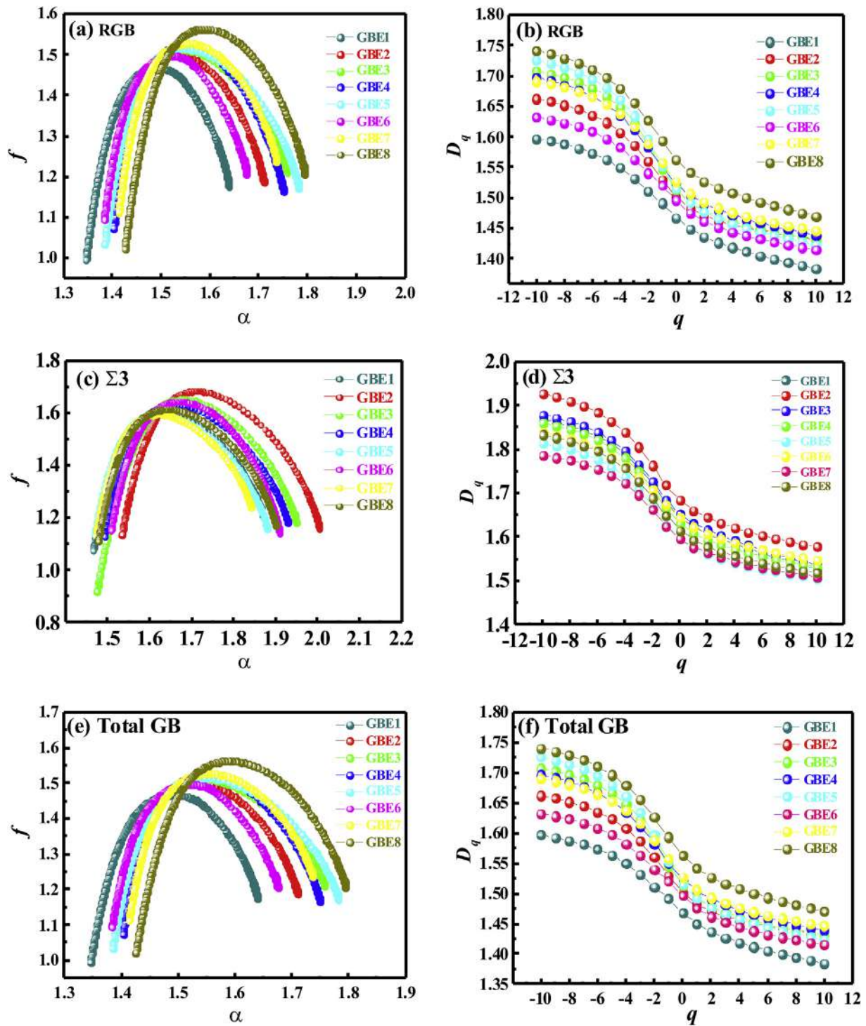
Fig. 9. Multifractal spectrum and generalized fractal spectrum of the RGB, \Sigma 3 GBs and total GB in the GBE (1–8) series samples; (a) (c) (e) multifractal spectra; and (b) (d) (f) generalized fractal spectra.
