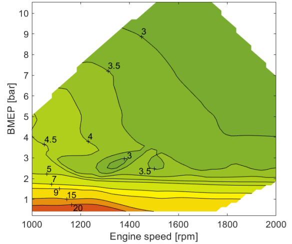
Figure 12: Specific NO emissions (g/kWh) as a function of engine speed and bmep at DO operation.
