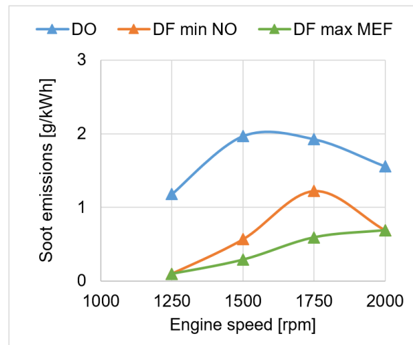
Figure 18: Specific soot emissions case study propeller curve.
