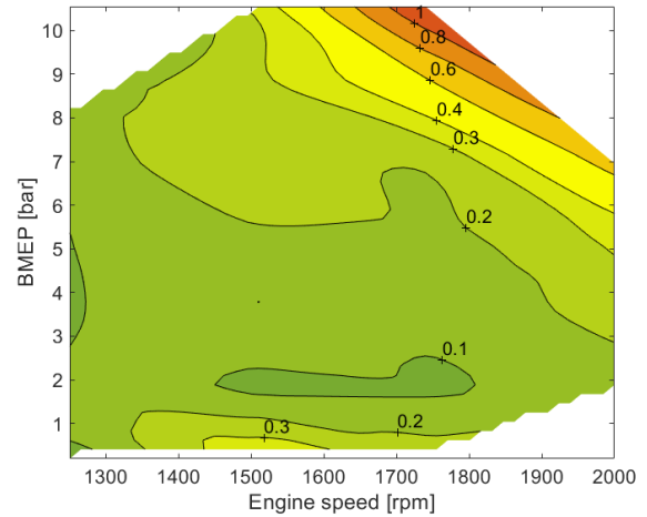
Figure 15: Specific soot emissions (g/kWh) in DF operation.
