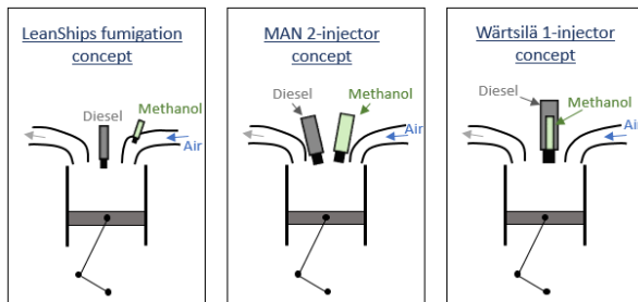
Figure 1: Overview of dual fuel methanol/diesel concepts demonstrated by LeanShips, MAN and Wärtsilä.
