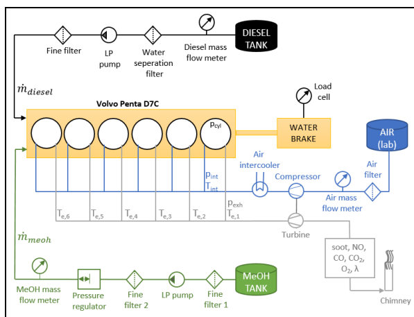
Figure 3: Test set-up showing the main gas and liquid flows to the engine, with the main components and measurement equipment.
