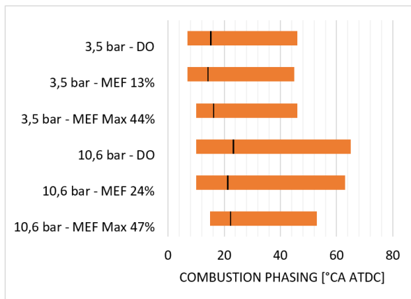
Figure 11: Combustion phasing for two different load points at 1500 rpm.
