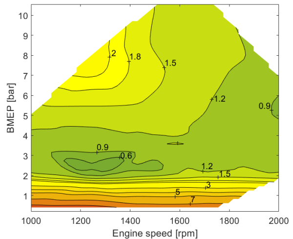
Figure 13: Specific NO emissions (g/kWh) as a function of engine speed and bmep at DF operation.
