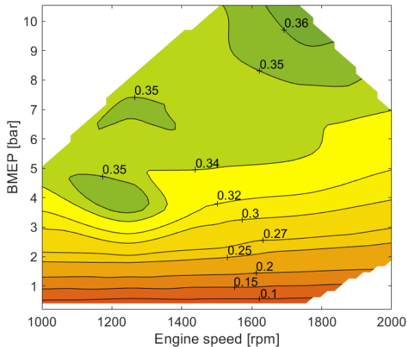
Figure 8: Brake thermal efficiency at DO operation.
