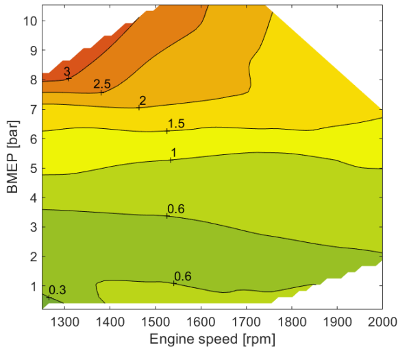
Figure 14: Specific soot emissions (g/kWh) in DO operation.
