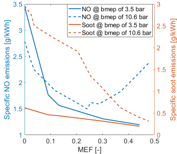
Figure 10: Specific NO and soot emissions as a function of MEF for two different load points at 1500 rpm.
