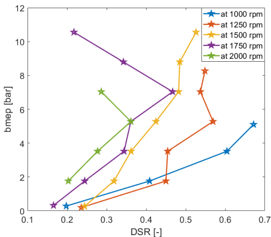
Figure 6: Maximum DSR as a function of load and engine speed.
