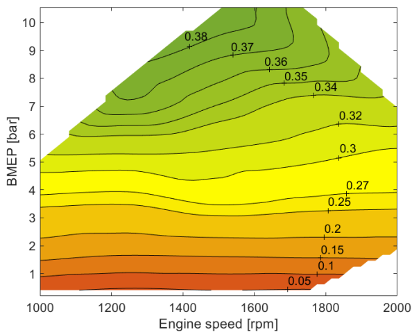
Figure 9: Brake thermal efficiency at DF operation at maximum MEF.
