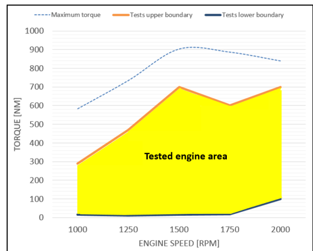
Figure 4: Tested engine area.
