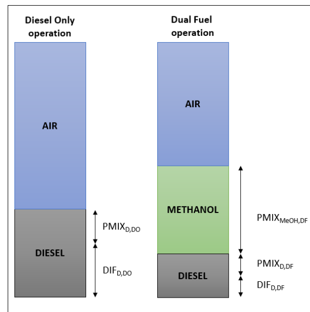
Figure 2: Fuel/air mass flow comparison between DO and DF operation, assuming equal efficiency in both operation modes and an eliminated diesel amount of 50% in DF operation. Ratios between DIF and PMIX (see text), and between fuel and air, are for illustrative purposes only.
