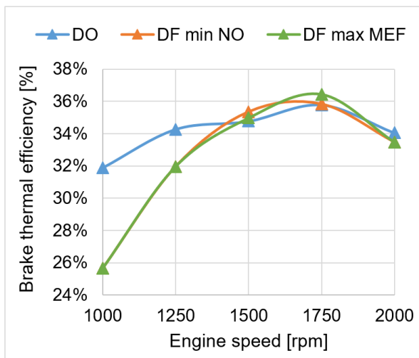
Figure 16: BTE for case study propeller curve.
