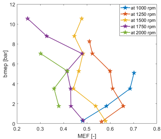
Figure 5: Maximum MEF as a function of load and engine speed.
