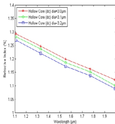
Fig 2. (a) The two dimensional end-face electric field distribution of the fundamental mode (b) Comparison between refractive Index and wavelength for hollow core diameter d_c=3 \mu\text{m} , d_c=3.10 \mu\text{m} and d_c=3.20 \mu\text{m} .
