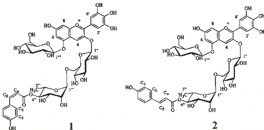
Figure 2. Structural formula of cis-Nasunin (1) and trans-Nasunin (2).
