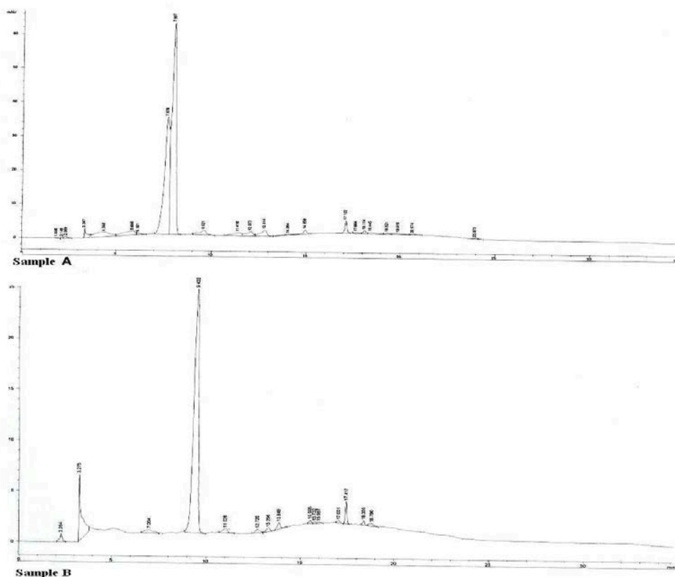
Figure 1. HPLC chromatograms of eggplant peels extracts of A solution (Panel A) and B solution (Panel B).
