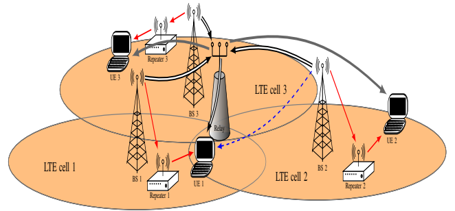
Fig. 1. Three overlapping LTE cells. The sum secrecy rates over the cells can be improved if a smart multi-antenna relay is introduced into the system. The emphasized arrows from BS 1 to the smart relay in the middle and then to UE 1 illustrate that desired signal strength (together with the direct channel path in red) can be boosted by choosing an appropriate relay strategy. The emphasized arrows from BS 2 to the smart relay and then to UE 1 illustrate that information leakage (shown by a dashed arrow in blue) can be neutralized by choosing the relay strategy appropriately.
