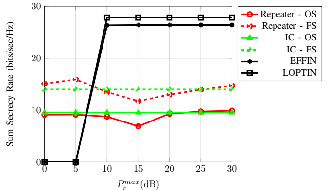
Fig. 5. The achievable sum secrecy rates of a two-user interference relay channel with 16 frequency subcarriers and 4 antennas at the relay is shown with varying relay power constraint. The TX power constraints are 10 dB and there are two antennas at the relay. The proposed scheme EFFIN and LOPTIN outperform baseline algorithms Repeater and IC by 200%. EFFIN achieves 94.86% of the sum secrecy rate performance by LOPTIN.
