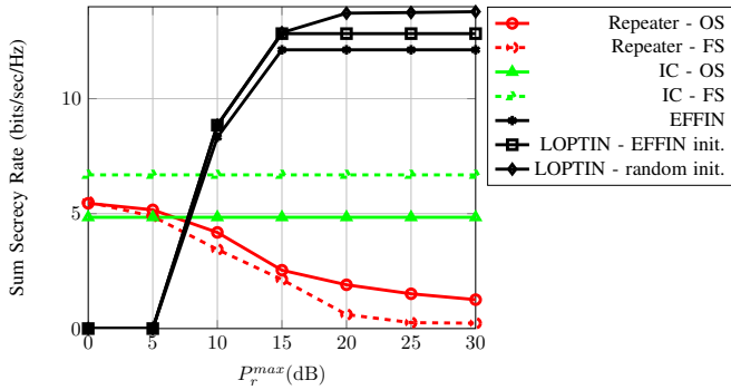
Fig. 3. The achievable secrecy rates of a two-user interference relay channel with 8 frequency subcarriers is shown with varying relay power constraint. The TX power constraints are 10 dB and there are two antennas at the relay. The proposed scheme EFFIN and LOPTIN outperform baseline algorithms Repeater and IC by 550% and 200% respectively.
