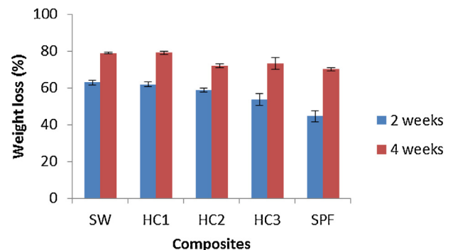
Fig. 6. Weight loss of Sw/SPF hybrid composites after soil burial for 2 and 4 weeks.
