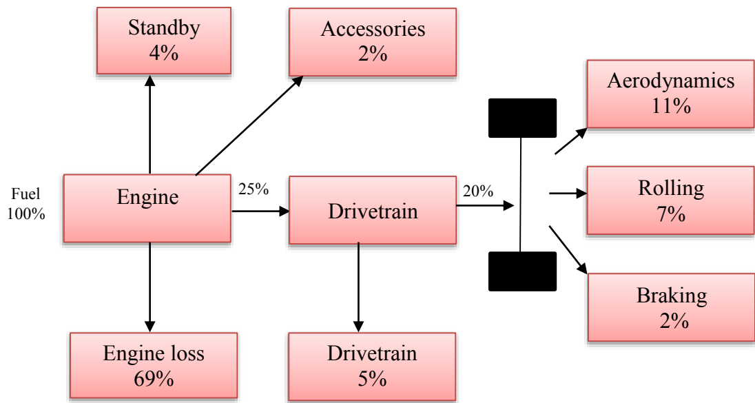
Figure 2.1 : Typical Fuel Energy Usage at Urban Driving
