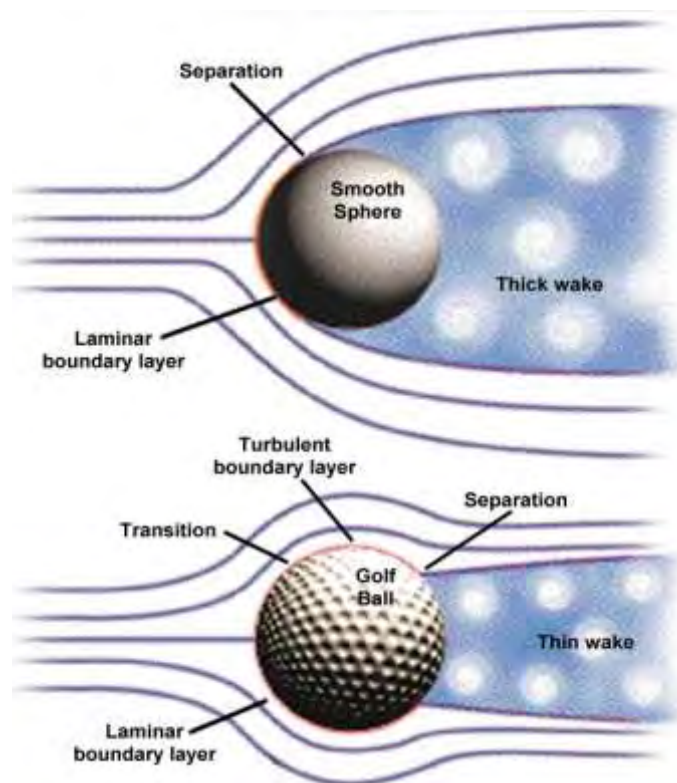
Figure 2.4 : Studied aerodynamics on golf ball (Alam et al., 2010)
