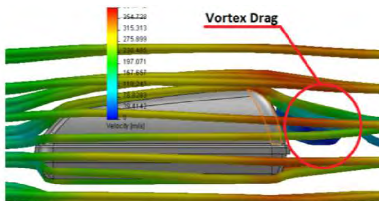
Figure 2.3 : Basic Flow Analysis on Roof Box using Solidworks
