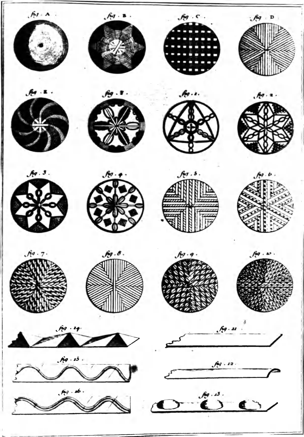
Plate 7. Maker of Embroidered Buttons, Diderot Button Plate 6.
