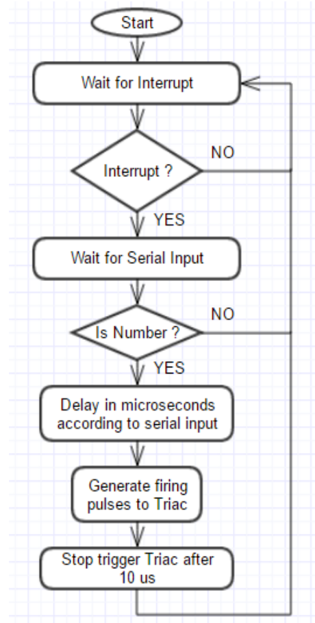
Figure 5: Arduino Coding Flow Chart
