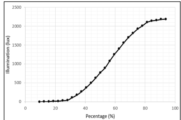
Figure 9: Illumination vs Percentage
