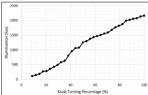
Figure 12: Illumination vs Knob Turning Percentage
