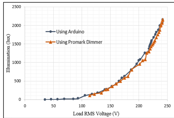
Figure 14: Illumination vs Load RMS Voltage
