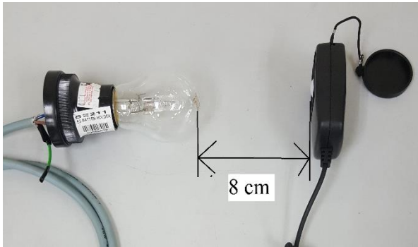
Figure 3: Illuminance of Lamp is measured by Lux Meter
