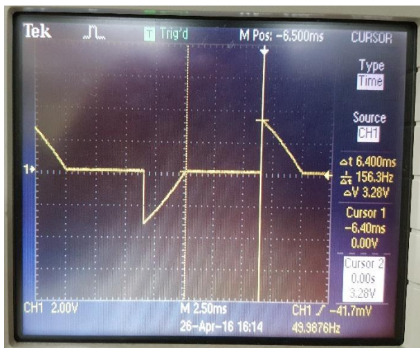
Figure 7: Measuring Exact Delay Time using Oscilloscope
