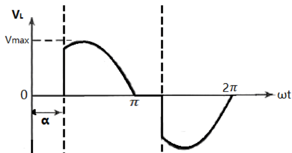
Figure 1: TRIAC Output Voltage Waveform
