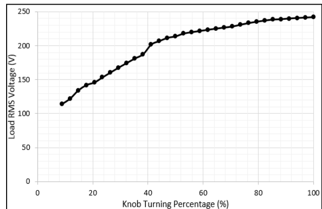
Figure 10: Load RMS Voltage vs Knob Turning Percentage
