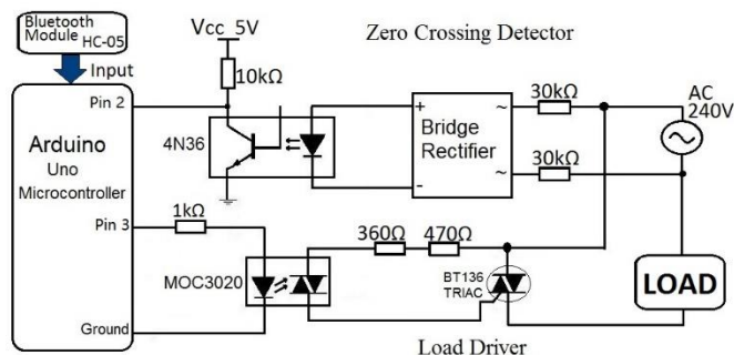
Figure 2: Phase Control Technique Circuit Diagram
