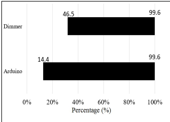
Figure 11: Comparison of Voltage Range Could Achieved
