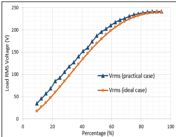
Figure 6: Load RMS Voltage vs Percentage
