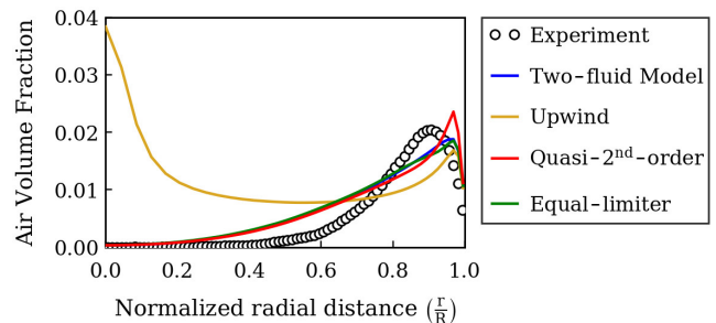
Figure 3: Radial profiles of the air volume fraction
