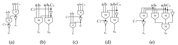
Fig. 5. Schematic diagrams of proposed 2-bit MLAFAs: (a) MLAFA11, (b) MLAFA22, (c) MLAFA12, (d) MLAFA21, and (e) MLAFA33.
