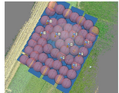
Figure 7. Project C, orientation of spherical and oblique images and extracted tie-points (sparse cloud).
