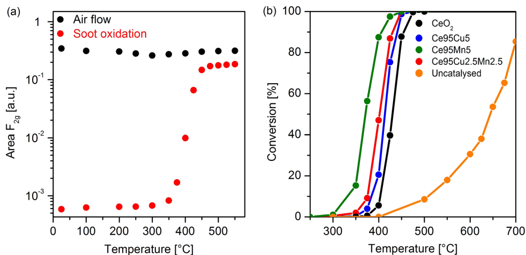
Figure 7. Variation of the F_{2g} peak area as a function of temperature during the analysis in air flow (black dots) and during soot oxidation (red dots) on the \text{CeO}_2 catalyst (a); the area of the F_{2g} band has been normalized to the acquisition parameters and to the area of the main band of the internal Si reference. Soot conversion curves obtained from the Raman spectra collected during the in situ tests over the four catalysts and for the uncatalysed reaction (b); the last curve was obtained as detailed in the caption of Supplementary Fig. S6.
