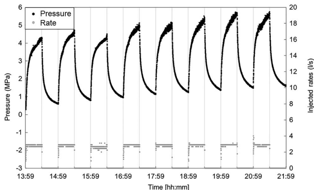
Figure 6. Pohang PX-1 pulse test HPT-1.
