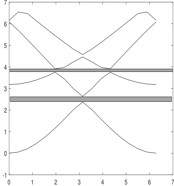
Figure 3: The perturbed dispersion curves and the band gaps shaded in grey
