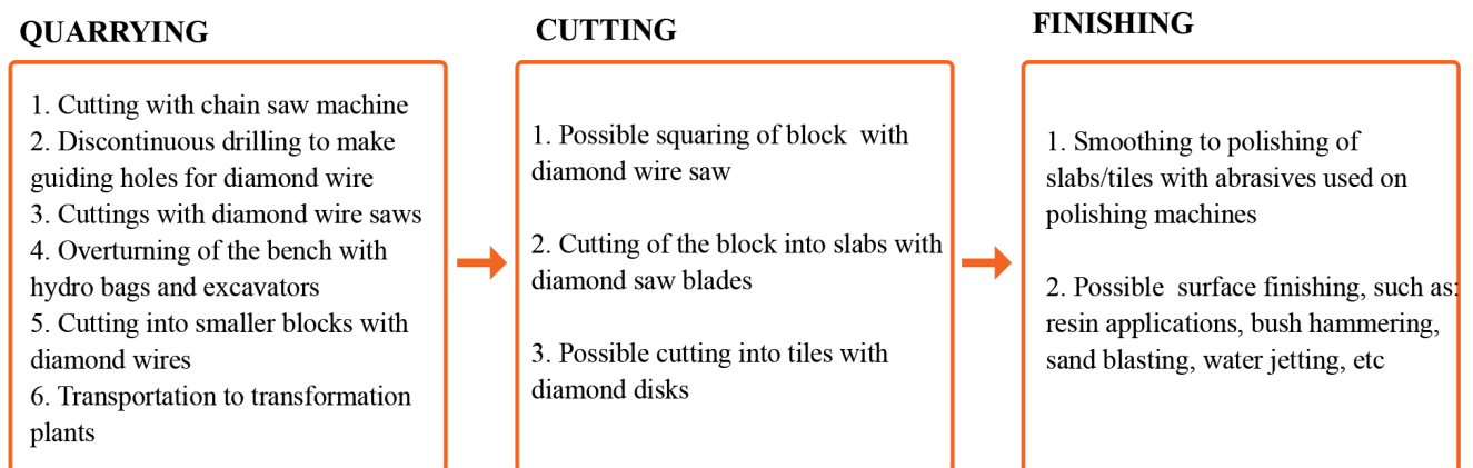
Fig. 2 - Scheme summarizing the techniques most commonly used in the Italian production chain of soft stone products (such as marble slabs and tiles)
