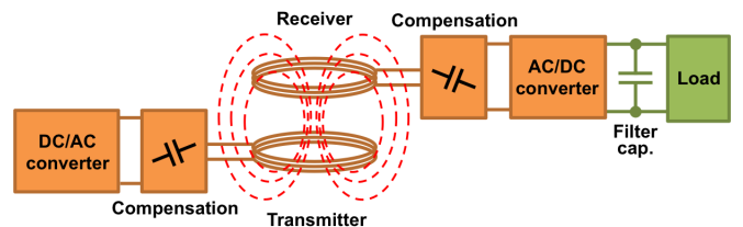
Fig. 1. General scheme of an IPT system.
