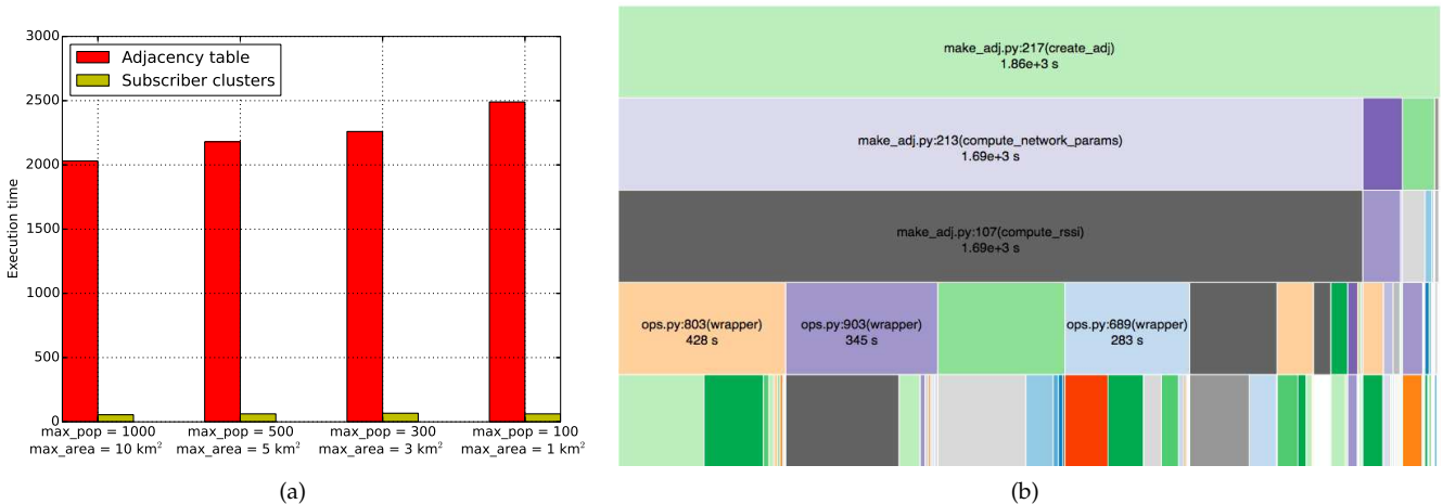
Fig. 5. Total time needed to create the weighed adjacency list and the subscriber clusters, for different values of the maximum population and area represented by each cluster (a); time breakdown when those limits are 1000 people and 10 km 2 respectively (b). Results have been obtained on a MacBook Pro equipped with a 2.7 GHz Core i5 processor and running OSX Yosemite.
