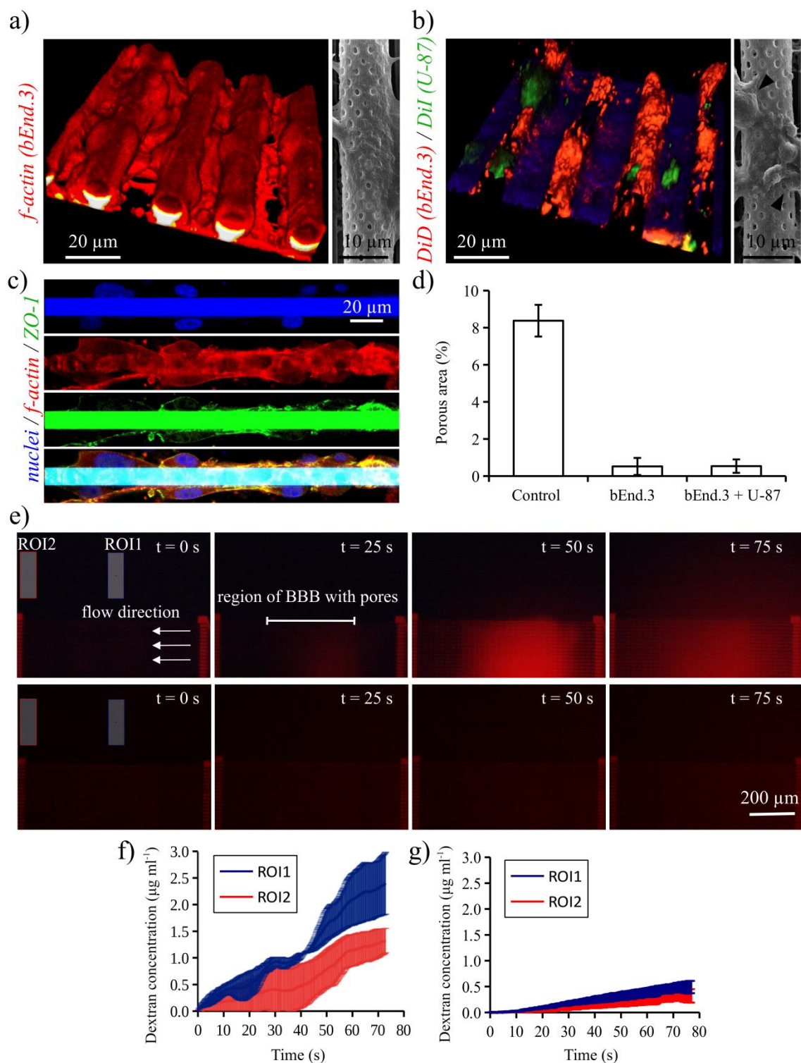
Figure 3. Dynamic 3D real scale bio-hybrid blood-brain barrier model. a) In the left image, the 3D rendering of confocal laser scanning microscopy (CLSM) showing bEnd.3 cells (f-actin in red) cultured covering the porous tubes of the microfluidic system; the right image shows a high magnification SEM image. b) Co-culture of endothelial-like bEnd.3 and human glioblastoma U-87 cells on the porous tubes of the microfluidic system; in the left image, the CLSM of bEnd.3 and U-87 cell membranes (shown in red and in green, respectively) and, in the right image, SEM image with black arrows indicating U-87 cells. c) Immunofluorescence staining against zonula occludens-1 (ZO-1), revealing a high expression of this marker (ZO-1
