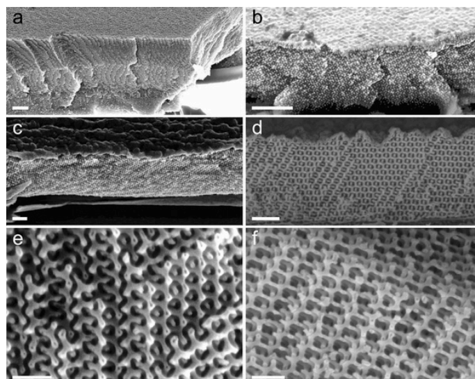
Figure 9. Side-view SEM images at a 45^\circ angle of gyroid replication into ZnO: (a) gyroid PS template; (b) as-deposited ZnO-PS hybrid; (c) ZnO gyroid after annealing at 550\text{ }^\circ\text{C} ; (d–f) different faces of the ZnO gyroid shown in (c). Scale bars are 1\text{ }\mu\text{m} for panels (a,b), 400\text{ nm} for (c,d), 200\text{ nm} for (e,f). Reproduced with permission from [124]; Copyright 2014 John Wiley & Sons, Inc.
