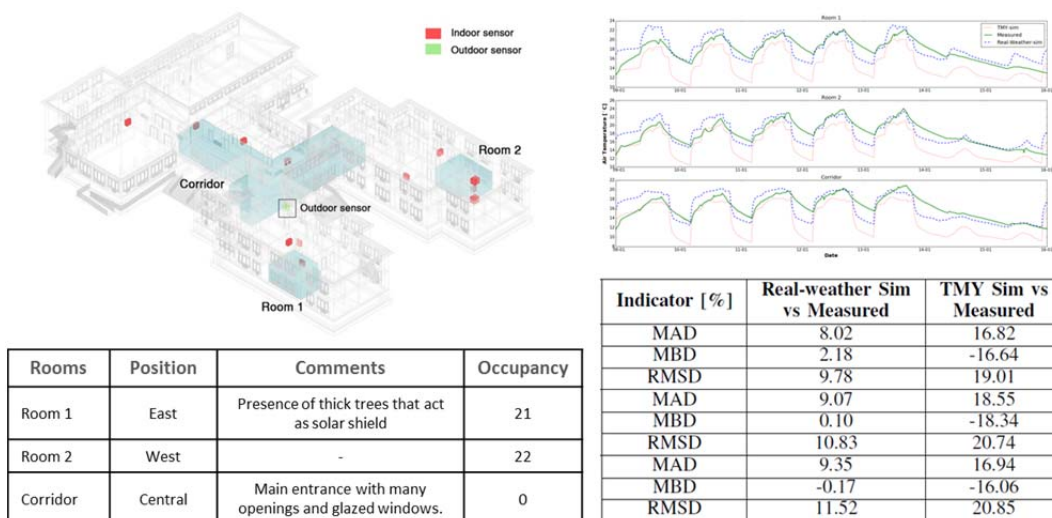
Figure 60: Simulated and measured indoor air temperature trends. EEB Project: Case study: Rodari school, modelled by Ossama Sabbar.
