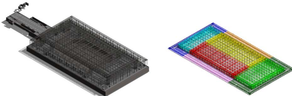
Figure 79: Thematisation of the steel structure by zones. Case study: Pala Alpitour, Turin.
