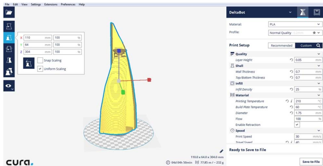
Figure 91: Cura interface and print setup. Case study: Menara TM, Kuala Lumpur.
