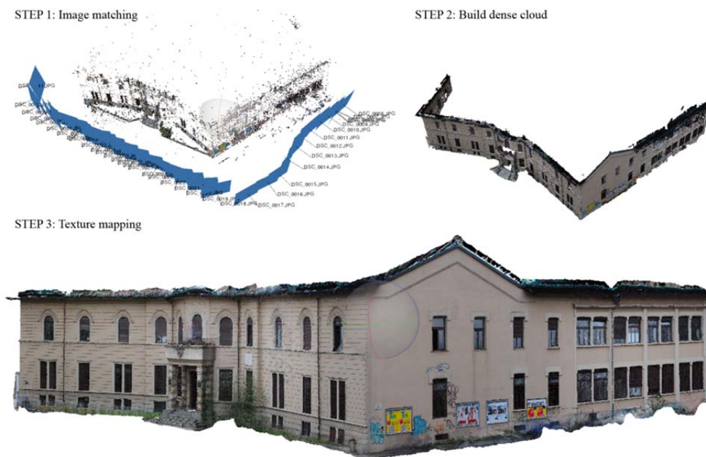
Figure 20: Point cloud realized with PhotoScan. TOBIM project. Case study: Corso Ferrucci 122.
