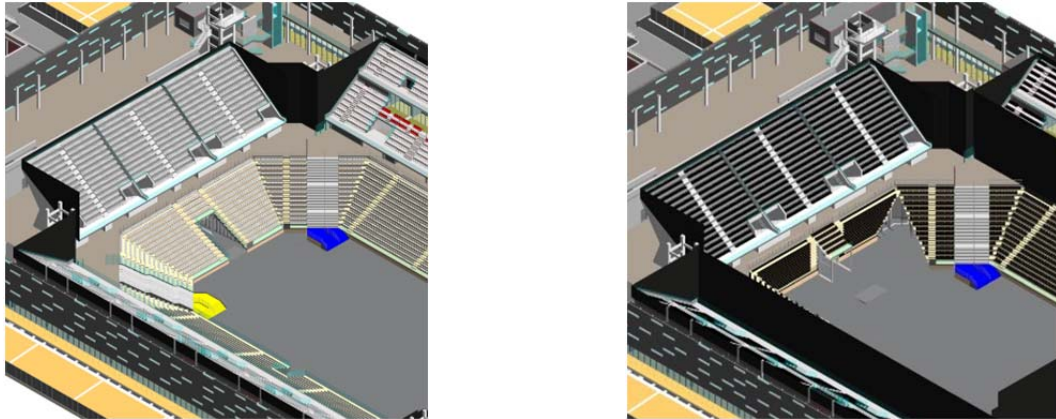
Figure 44: Configuration scenarios evaluation through the BIM model.
