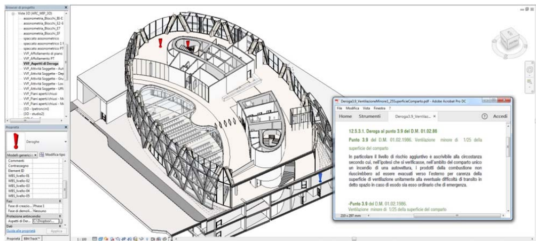
Figure 70: Aspects of derogation through customized family.
