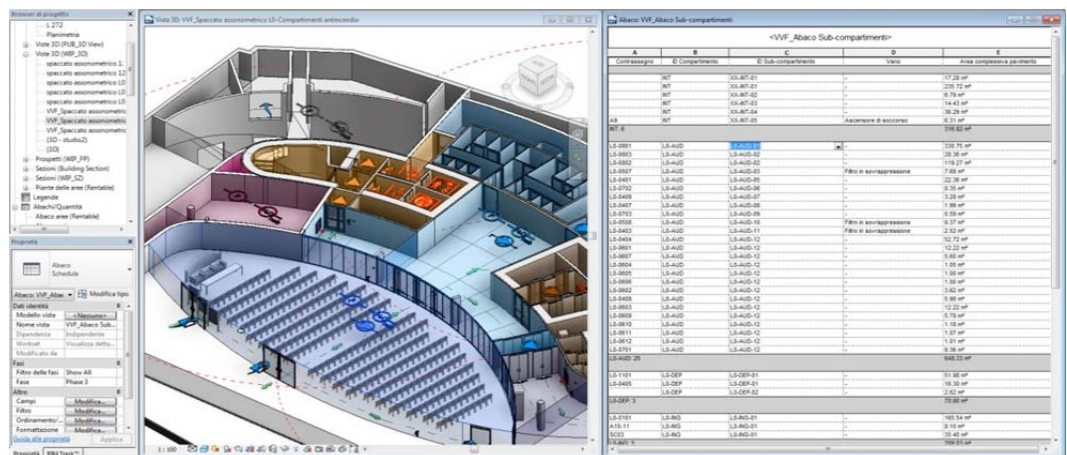
Figure 66: Fire compartments and systems installed schedule.
