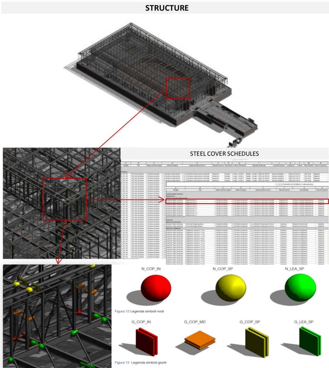
Figure 83: Nodes and connections implementation and management.
