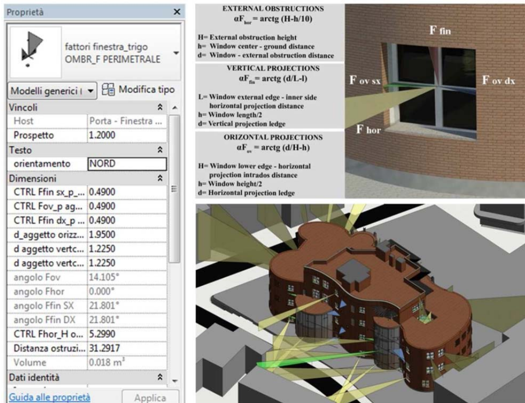
Figure 56 Surface-based Revit family for shading values calculation. EEB Project. Case study: Biblioteca Archimede, modeled by Maurizio Dellosta.
