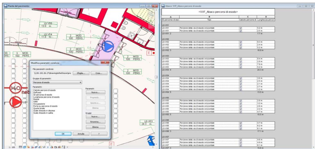
Figure 67: Escape routes objects and parameters.
