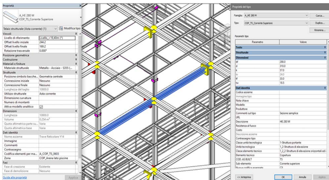
Figure 81: parametric modelling of steel structural auctions.
