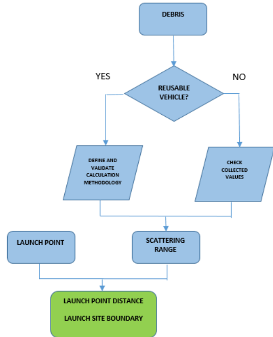
Fig. 7: Spaceport area restriction evaluation flow
