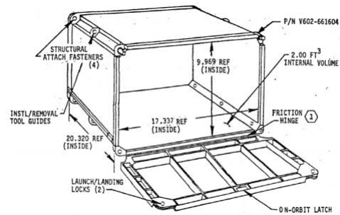
Fig.4: NASA Space Shuttle Middeck Locker Dimensions (Source: NSTS-21000-IDD-MDK)
