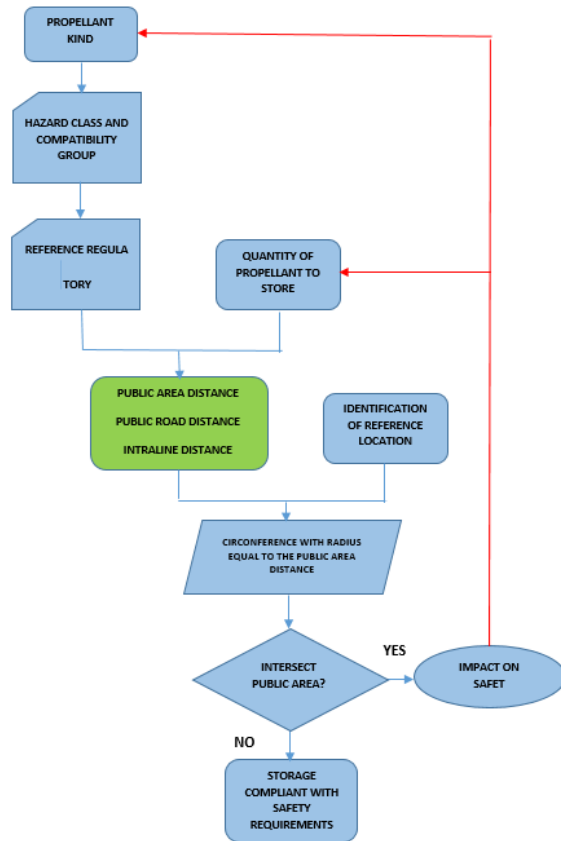
Fig. 8: Maximum propellant storage evaluation flow
