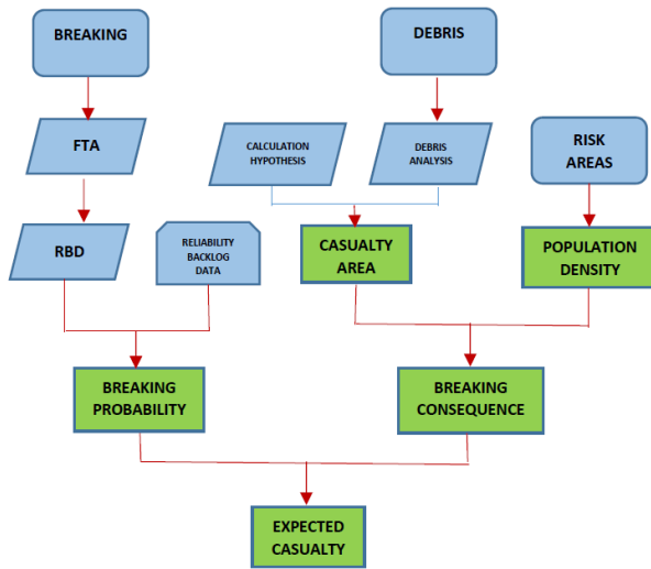
Fig. 6: Expected casualty evaluation flow chart
