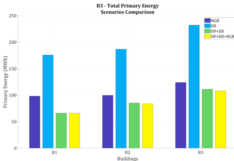
Fig. 8. Scenarios comparison: Total Primary Energy consumption in the analyzed buildings.
