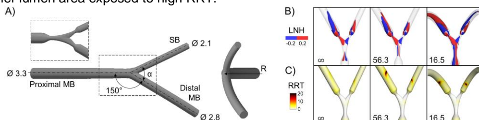
Figure 1 – A) Parametric coronary bifurcation model. Diameters are in mm. B) Isosurfaces of local normalized helicity (LNH); positive/negative values of LNH indicate counter-rotating flow structures. C) Contour maps of relative residence time (RRT).
