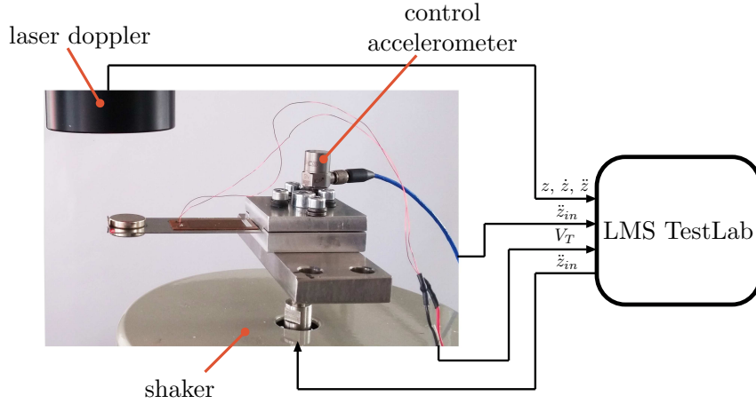
Fig. 6.6 Experimental setup.
