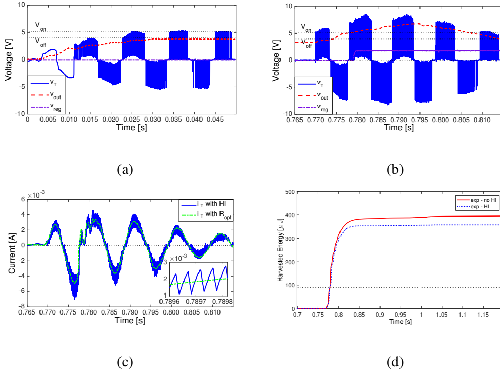
Fig. 5.33 Experimental voltages a) during the first step and b) during the second step, with \alpha = 2 and T_{delay} = 20 \mu s . c) Experimental currents during the second step with the HI shown together with the experimental current in optimal resistive load condition. d) Harvested energy during the second step.
