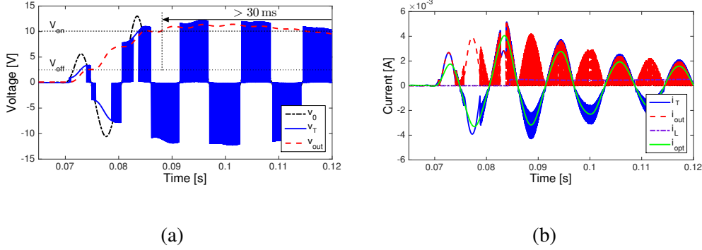
Fig. 5.18 Waveforms of a) voltages and b) currents defined in Fig. 5.15 assuming \alpha_{HI} = 2 and T_{delay} = 20 \mu s .
