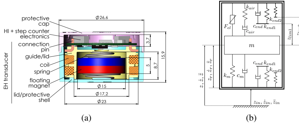
Fig. 5.3 EH Bluetooth step-counter layout: main components and dimensions in mm.
