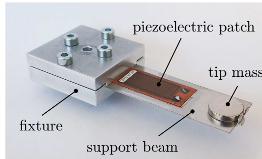
Fig. 6.1 Piezoelectric EH prototype.
