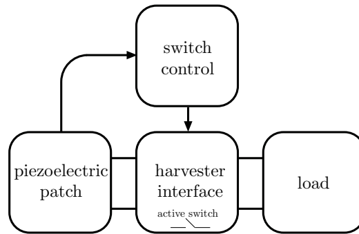
Fig. 6.14 Piezoelectric EH embedded with self-powered synchronized switching interface.
