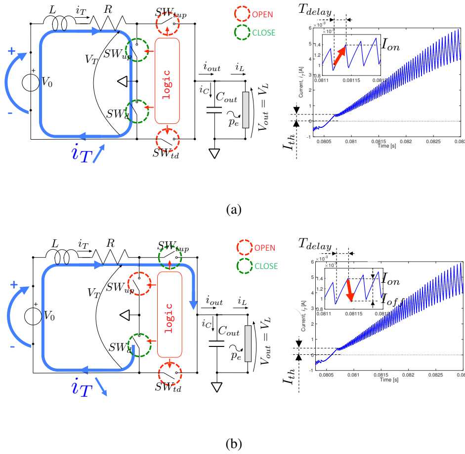
Fig. 5.16 HI working principle: a) energising and b) transferring phase.
