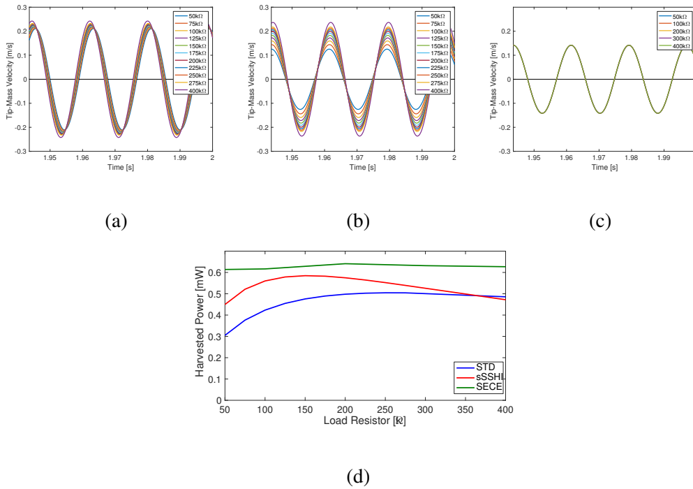
Fig. 6.18 Numerical comparison among STD, sSSH and SECE interfaces. Tip mass velocity in the case of a) STD, b) sSSH and c) SECE interface for different load resistor values. d) Harvested power as a function of R_L .
