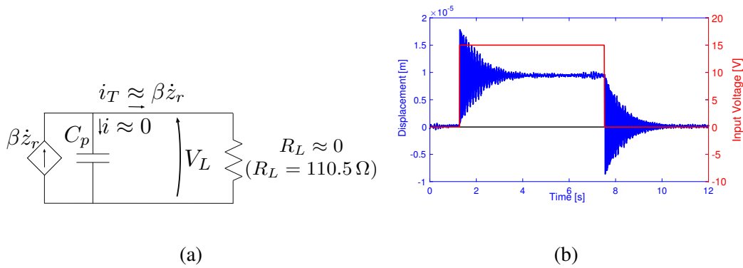
Fig. 6.12 a) Electric scheme for \beta coefficient evaluation. b) Mechanical response to imposed voltage.
