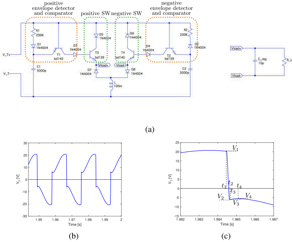
Fig. 6.16 sSSH technique: a) electrical scheme and b)-c) V_T in response to 2 \text{ m/s}^2 56.2 Hz sinusoidal input with R_L = 50 \text{ k}\Omega .
