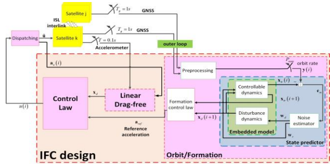
Fig. 3. Overall scheme of the IFC control unit.
