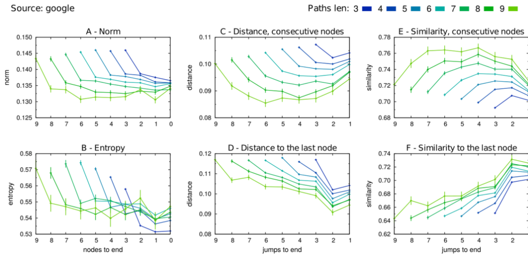
Fig. 4.5 Paths generated from the external source google : averages. The 10^7 paths simulated with google as source were split by lengths. For each fixed length l , the averages of the following quantities were computed over all the nodes(pairs) at k steps(jumps) from the end: (A) the average norm \overline{\|w_k^l\|} , (B) the entropy \overline{S(w_k^l)} , (C) the distance and (E) the similarity between all the pairs of nodes consecutively visited along each path, respectively \overline{d(w_k^l, w_{k-1}^l)} and \overline{sim(w_k^l, w_{k-1}^l)} , (D) the distance and (F) the similarity between every node visited and the ending node along each path, i.e. \overline{d(w_k^l, w_0^l)} and \overline{sim(w_k^l, w_0^l)} . The error bars display the standard errors of the means. Each color refers to a path length, from 3 (blue) to 9 (light green).
