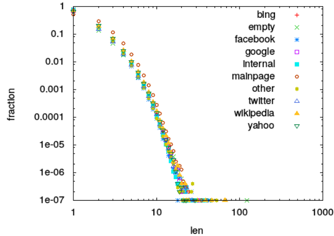
Fig. 4.2 Distribution of the path lengths. For the 10 different external sources, the average distributions of the lengths of the simulated walks are reported. The averages are performed over 10^7 simulations for every source.
