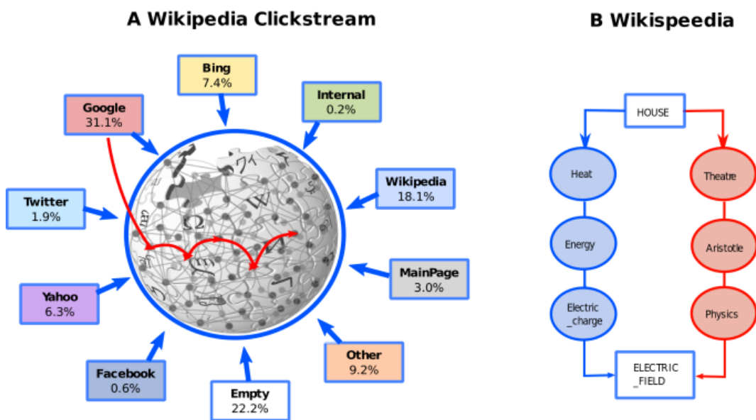
Fig. 4.1 Datasets under consideration. In (A) the English Wikipedia Clickstream dataset is illustrated. The 9 different external sources plus the MainPage are displayed with the fraction of flux outgoing from them. The paths considered in the present analysis start from one of the 9 sources to randomly walking over the Wikipedia articles accordingly to the transition counts provided by the dataset. As an illustration, in red line a decorative path starting from Google and them jumping on different pages of the Wikipedia graph is reported. (B) Two examples of paths followed by players of the Wikispeedia game, whose task was that of navigating on a reduced version of Wikipedia from a given starting page to a given target one (from House to Electric_Field in the example).
