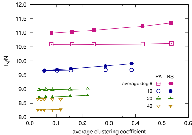
Fig. 3.5 Coverage times and graph transitivity. The figure shows the average coverage times scaled to the network order ( N = 10^4 ) obtained on scale-free graphs generated according to the model proposed by Holme and Kim [63] as functions of the average clustering coefficient. Different colors refer to graphs with different minimum (and thus also average) degree, while empty or filled symbols distinguish data obtained when respectively the PA or the RS entry selection criterion is used.
