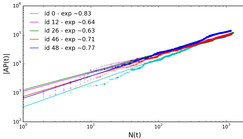
Fig. 5.17 Adjacent possible expansion as a function of the number of tags introduced. For the five longest textbooks, the cardinality of the adjacent possible is reported as a function of the number of distinct units introduced N(t) , corresponding to |\mathcal{A}(t)| , after averaging over the different stream realizations. For each textbook, the average curve is fitted via a power-law function AP(N) = aN^\beta , via least square method. The resulting fitted curves as well as their exponents are also displayed.
