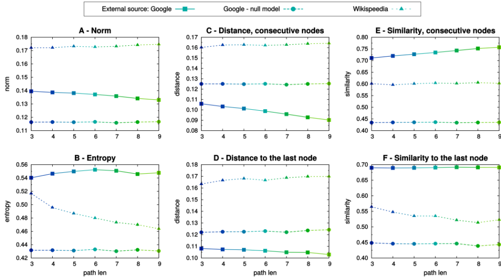
Fig. 4.6 Averages over the aggregated paths. The averages of measures already introduced in Fig.4.5 are here computed over all the nodes encountered along walks of fixed length l . Squares, circles and triangles refer respectively to the paths generated from the source google , to the same paths but semantically reshuffled (null model) and on the paths generated in the Wikipedia game. Using the same palette of Fig.4.5, each color refers to a length. The standard errors of the means are reported, though not visible at this scale.
