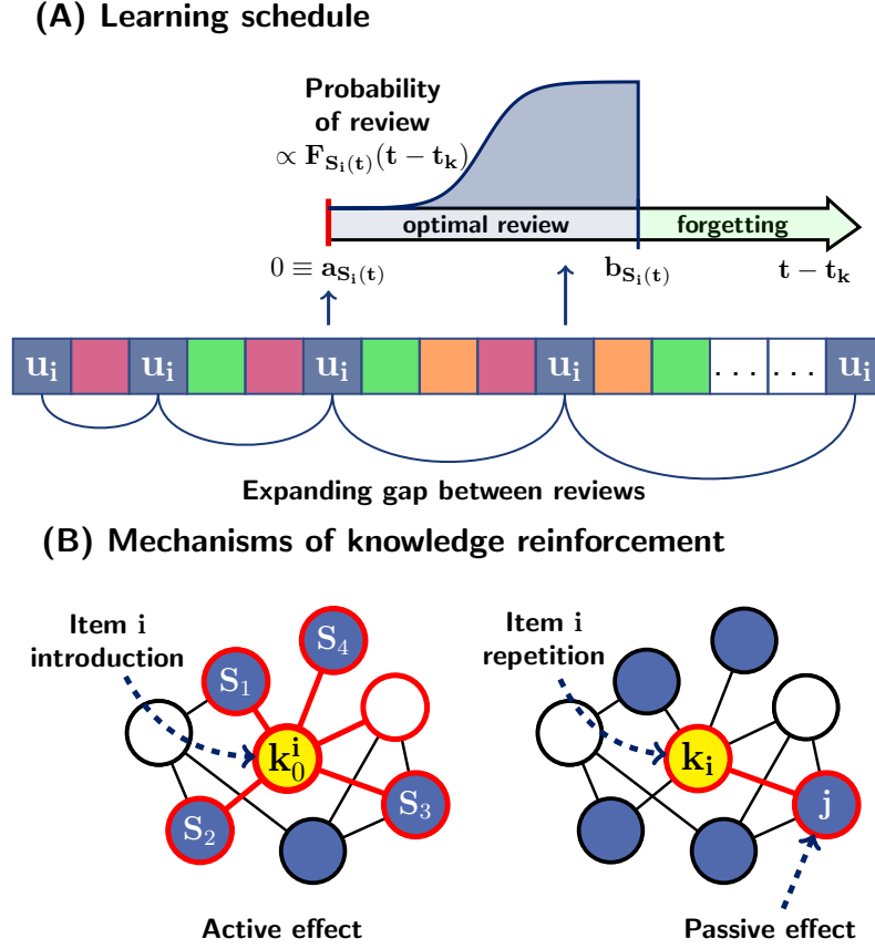
Fig. 3.1 Model illustration. (A) In a learning schedule the interval required between any two successive presentations of the same item i expands with the number of reviews. To this end the probability of a repetition is computed for every node already introduced as illustrated. If the k -th presentation of a node i with knowledge strength S_i occurred at time t_k , the (k + 1) -th happens at time t with probability proportional to F_{S_i(t)}(t - t_k) . This function is non null in the temporal interval [a_{S_i(t)}, b_{S_i(t)}] , whose bounds are increasing functions of the total knowledge strength of item i . After b_{S_i(t)} steps without being repeated, the item i is forgotten and has to be reintroduced. In (B) the supposed mechanisms of knowledge reinforcement are illustrated. When item i is introduced, it gains a starting knowledge value k_0^i depending on how much its neighborhood is known. This mechanism is referred to as active effect . Afterwards, at every successive repetition, its knowledge is reinforced by 1 and one among its introduced neighbours, say j , is randomly selected to receive a passive reinforcement, i.e., k_j^{pass} is incremented by a quantity \alpha . In all the simulations here conducted \alpha = 0.1 .
