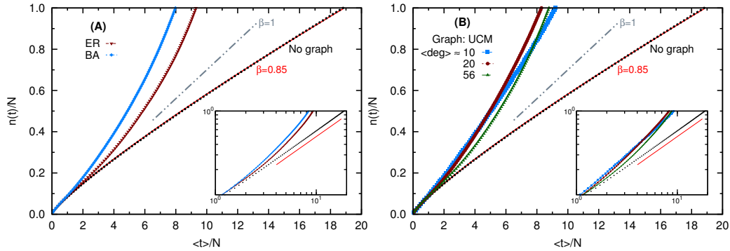
Fig. 3.6 Introduction rate on synthetic graphs. Fraction of distinct nodes introduced as a function of the (rescaled) average time needed to cover them. In figure (A) we report data obtained on Erdős-Rényi model [42] and Barabási-Albert model [14] graphs with average connectivity \langle deg \rangle \sim 100 . In (B) the graphs considered are generated according to the uncorrelated configuration model [28] with P(deg) \propto deg^{-\gamma} and \gamma = 2 and different average connectivities. In all the cases, the graph size is N = 10^4 and the algorithm used to select the entries is the random surfing RS. In both (A) and (B), with black dots we report the introduction rate for an equivalent set of uncorrelated items. It is fitted with a sub-linear curve y \propto x^\beta , with \beta = 0.85 . The fitting curve is shown with red line in the main graph, while in the insets we report an eye-guide power-law with same exponent. An eye-guide linear ( \beta = 1 , grey line) curve is also reported in the main figures. The insets axes are in log-log scale. The data are averaged over 50 agenda simulations. Standard errors are reported, though not visible at the plot scale.
