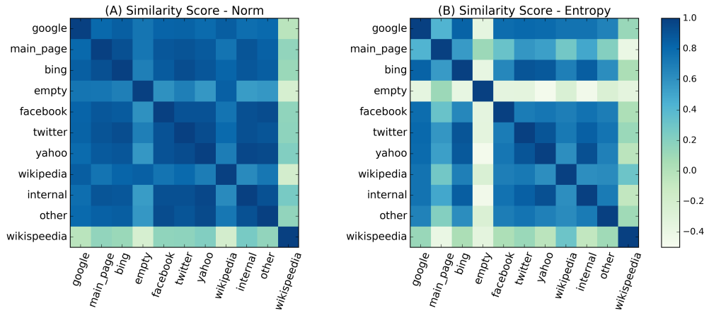
Fig. 4.9 Similarity scores between sources. For the two observables norm (left panel) and entropy (right panel), we report the matrix of similarities score between all the sources and Wikispeedia. The score is defined by equation 4.6 and eq. 4.7. For each pair of sources, the unrescaled averages values of the observable are considered (as in Fig. 4.5). Then, for each path length between 4 and 9, the spearman correlation coefficient is computed between the averaged values of the observable. The final score is the obtained after averaging over all the lengths.
