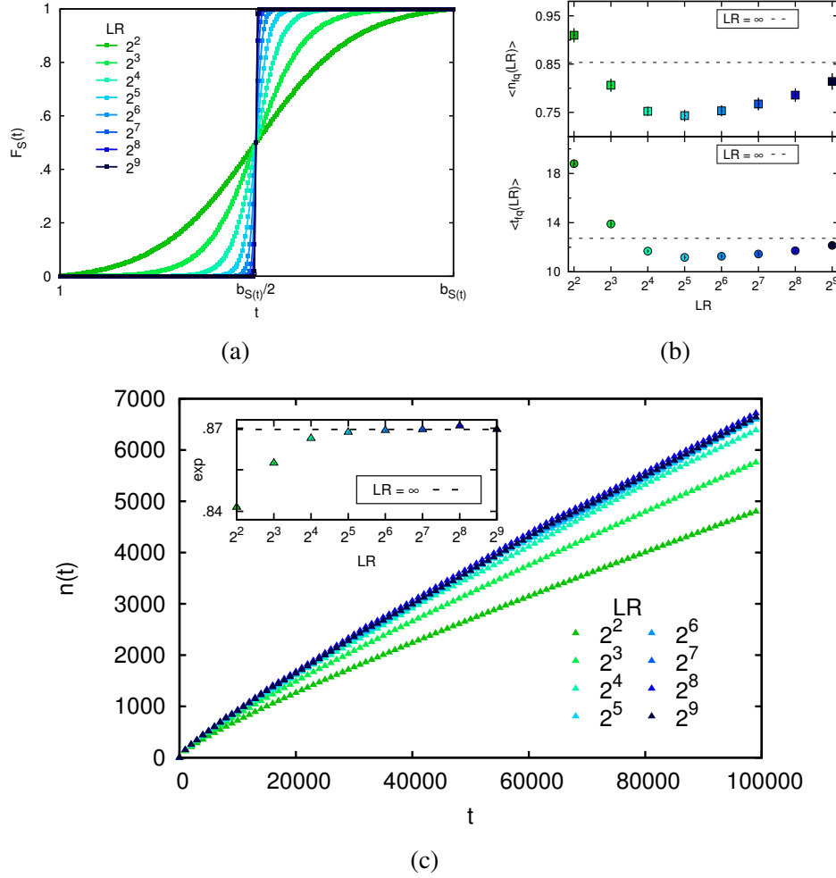
Fig. 3.2 Learning rigidity and schedule efficiency. In (a), different plots for the function F_{S_i}(t) (Eq. 3.3) in the interval [0, b_{S_i}(t)] are reported, while tuning the value of the parameter LR . Correspondingly, in the figures (b) and (c) some properties of the agendas obtained by running the simulations on sets of 10^4 disconnected nodes are displayed. In particular, in (b) it is reported the average number of units in the forgetting queue (subfigure at the top) and the average number of time steps a forgotten unit has to wait before being reintroduced (bottom). In (c) the introduction rates n(t) are reported, with the exponent of the fitting function n(t) \propto t^{exp} in the inset. All the data are averaged on 50 runs. Standard errors are reported.
