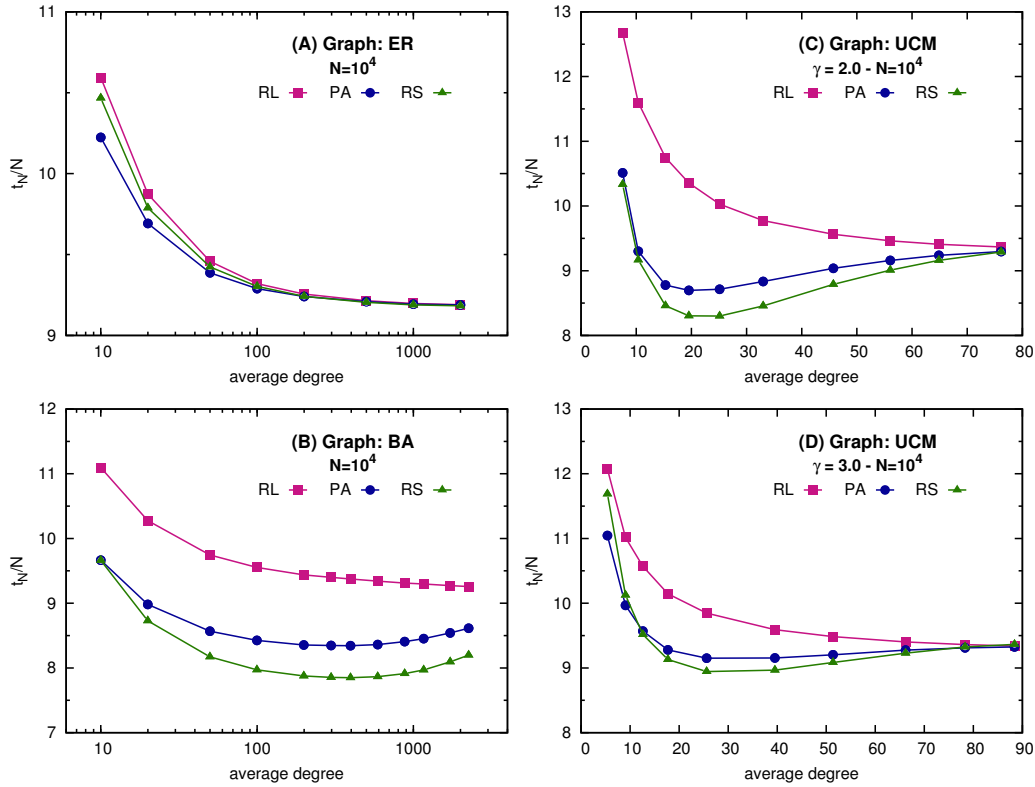
Fig. 3.4 Coverage times on synthetic graphs. In the figures, the mean coverage times scaled to the network order N = 10^4 as a function of the network average degrees are shown for different synthetic graphs, generated according to the (A) Erdős-Rényi model [42], (B) Barabási-Albert model [14], (C) uncorrelated configuration model [28] where P(deg) \propto deg^{-\gamma} and \gamma = 2 , (D) same as in (C) with \gamma = 3 . The data are averaged over 10 different graph realizations and 5 learning agendas for each of them. Standard errors are also reported but they are covered by symbols. Different colors refer to the three criteria used to select the entries: random learning (RL, magenta), preferential acquisition (PA, blue) and random surfing (RS, green). Note the logarithmic scale of the horizontal axis for (A) and (B).
