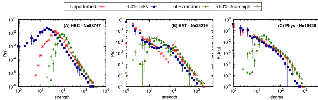
Fig. 3.3 Strength and degree distribution for original and perturbed real graphs. data are displayed which refer to (A) HBC graph, (B) EAT graph and (C) Wikipedia Physics subsection graph. Red symbols refer to the unperturbed graphs. Starting from each unperturbed structure, 50% of links were randomly removed (blue squares), randomly added (filled green circles) or randomly added only between second neighbours (empty green triangles). The data are averaged over 10 different realizations of each perturbation procedure. Standard deviations are shown.
