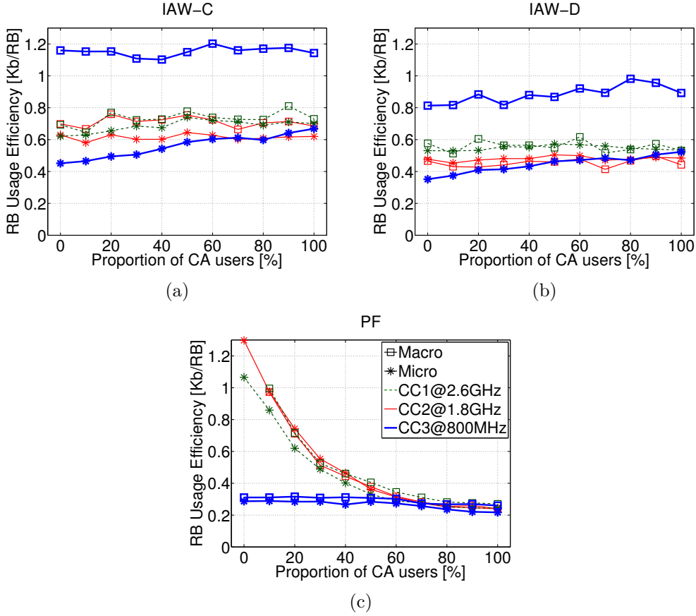
Figure 5.8. RB usage measured in Kb/RB for each CC: (a) IAW Centralized; (b) IAW Distributed; and (c) Proportional-Fair. The legend for all there subfigures is shown in the top right-hand corner of subfigure (c). We differentiate between different types of BSs using different markers, and between different CCs using different line styles and colours.
