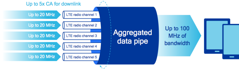
Figure 2.2. Carrier aggregation concept: several component carriers are used simultaneously to provide more bandwidth to the end user [25].
