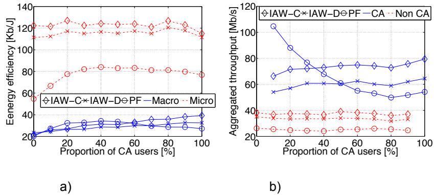
Fig. 5. a) Energy efficiency measured in Kb/J for macrocells (blue/solid line) and microcells (red/dashed line); b) average aggregated user throughput in Mb/s for CA users (blue/solid line) and legacy users (red/dashed line). We differentiate between the different algorithms using different markers.
