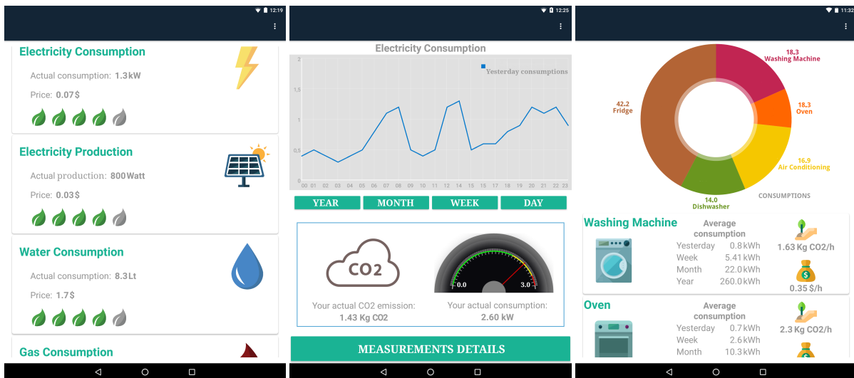
(a) Main Activity (b) Consumption Activity (c) Detailed Consumption Activity Figure 4: Example of activity views visualized with the Android mobile application
