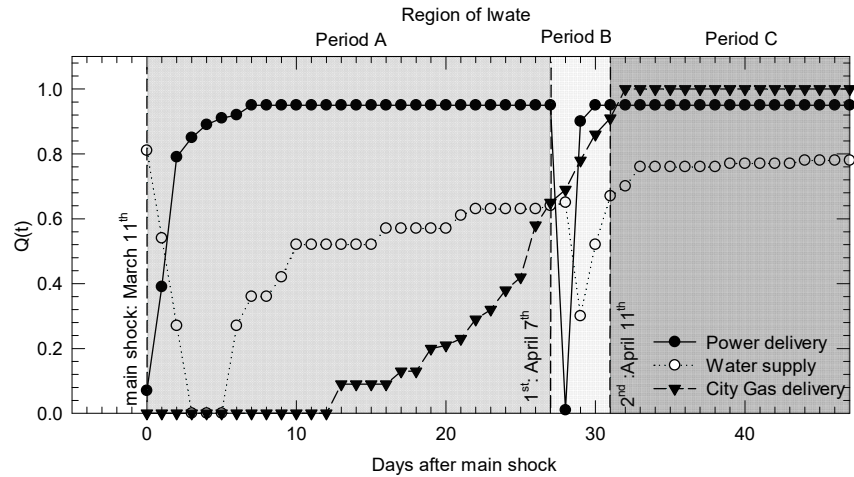
Figure 4 Restoration curves of Iwate region with subdivision into homogeneous parts between two consecutive strong shocks
