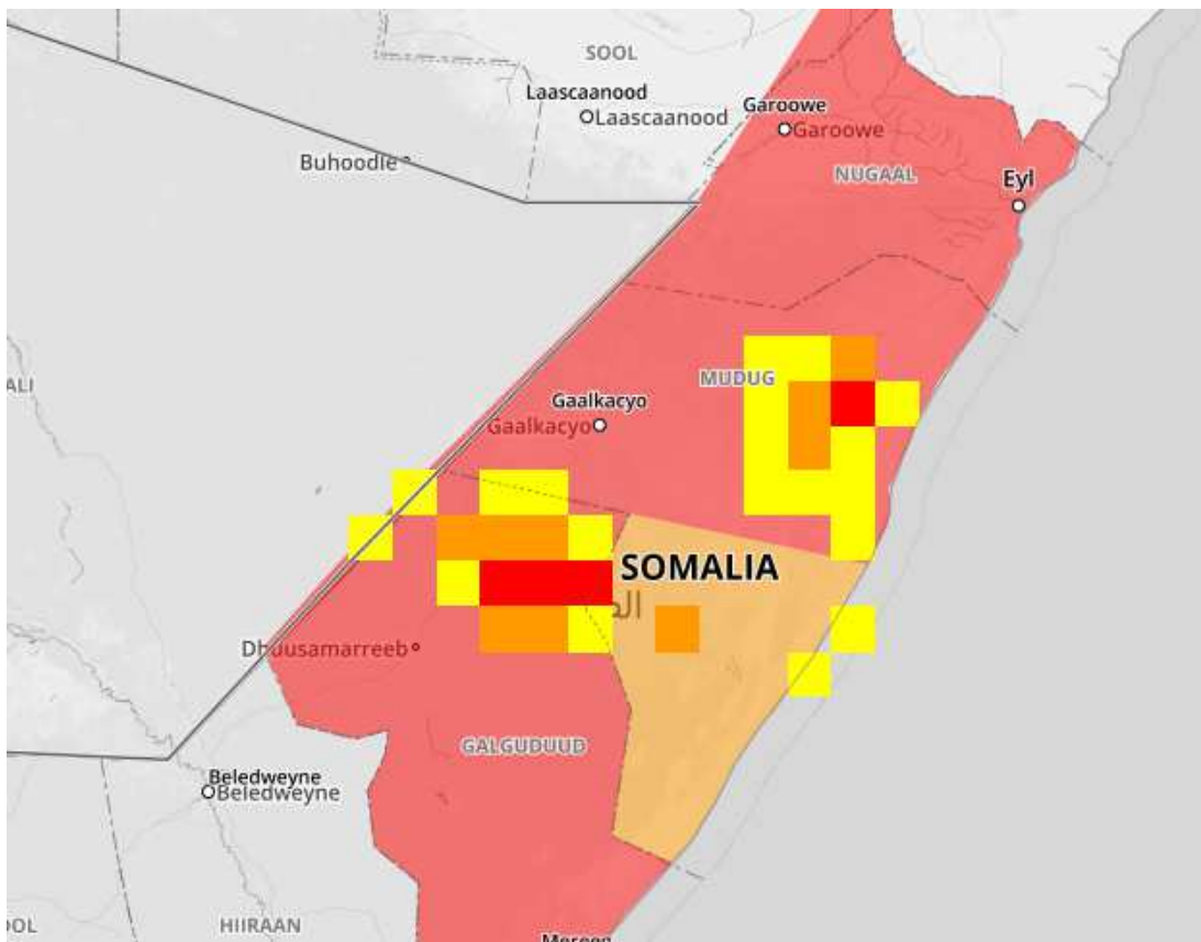
Figure 5.9 alert near real-time at pixel scale superposed to alert districts 48h (zoom over Somalia 08/05/2016)
