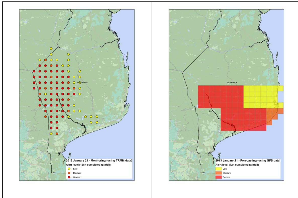
Figure 5.4 Situations as of January, 21 th . a) On the left: alerts about accumulated rainfall over the past 7 days; b) on the right: alerts about accumulated forecasted rainfall for the next 3 days.
