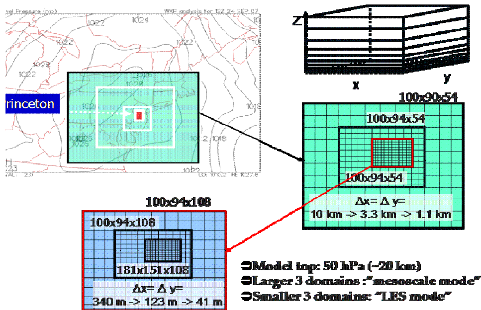
Figure 3.1 Initialization of a mesoscale model with a global model (source http://efm.princeton.edu/ )
