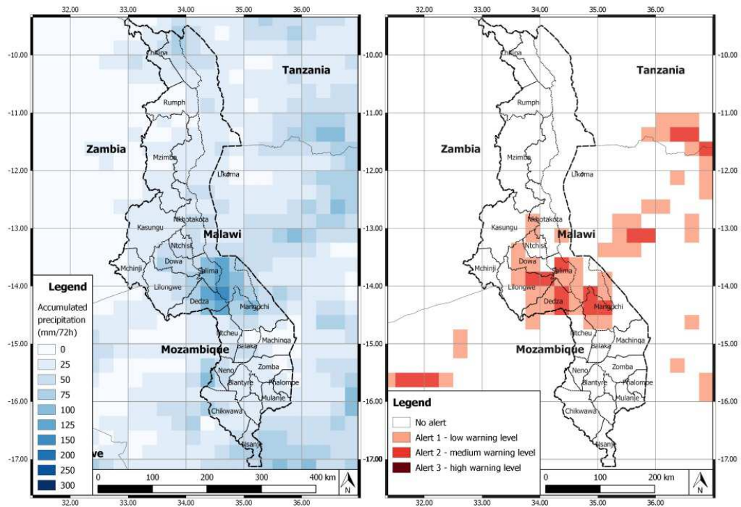
Figure 5.10 72h TRMM-3B42RT accumulated precipitation and Extreme Precipitation Alerts (05-07 January 2013)
