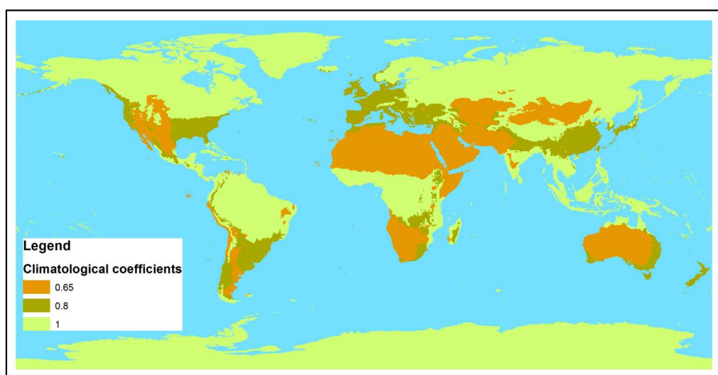
Figure 5.2 - Climatological coefficients for the calculation of fixed rainfall thresholds.
