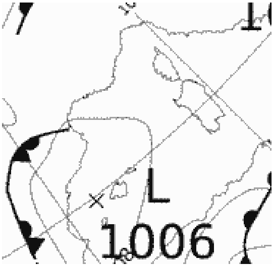
Analysis 02.00LT (00.00UTC)
