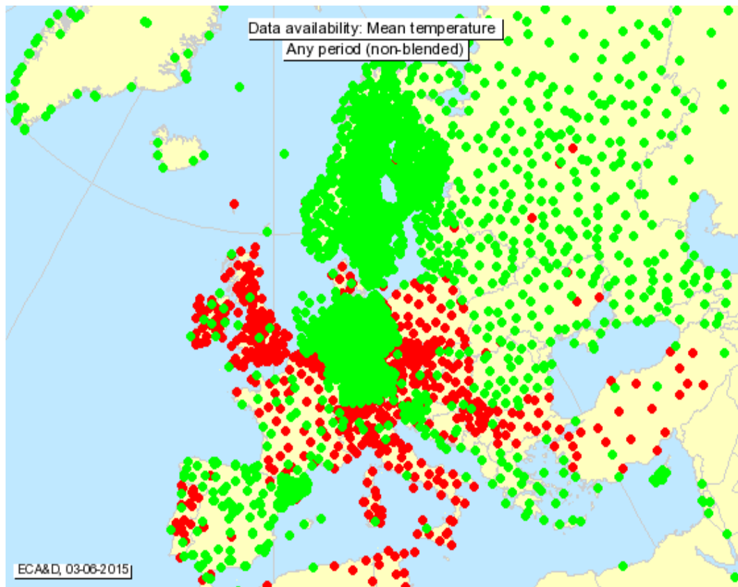
Figure 3.6 Mean Temperature data availability in Europe ( http://variable-variability.blogspot.it/2015/06/congress-WMO-free-climate-data.html )
