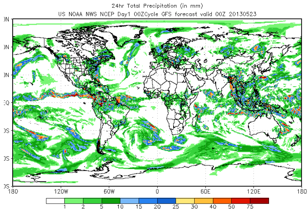
Figure 3.2: The cumulated GFS raster (source catalog.data.gov)
