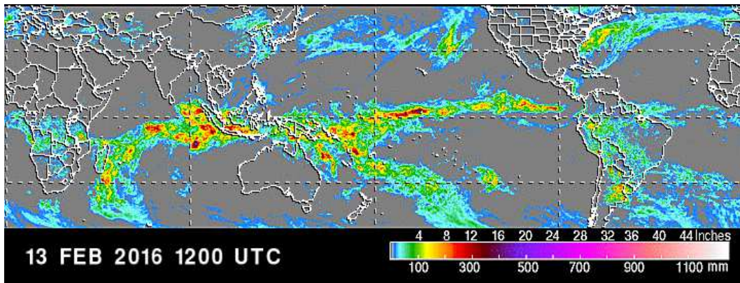
Figure3.3 accumulated precipitation from TRMM (source trmm.gsfc.nasa.gov/)
