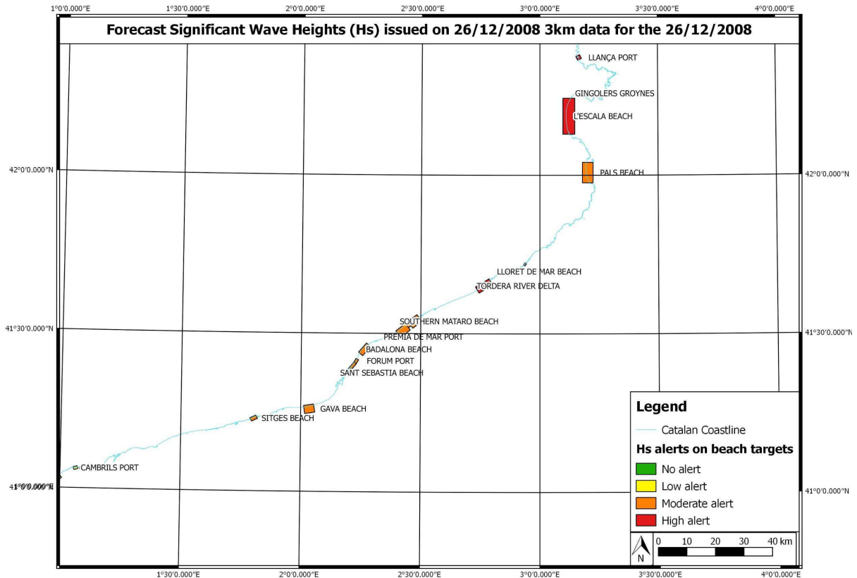
Figure 5.14 Example of alerts estimated for the Catalan beach targets regarding the Hs CSI (forecast WRF 3km issued on 26/12/2008 for the 26/12/2008).
