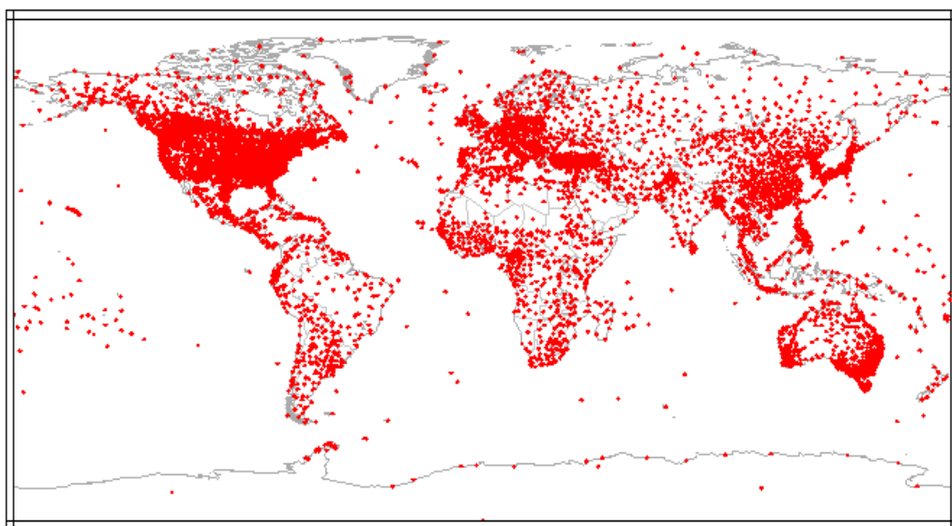
Figure 3.4 Map of land stations in the Global Historical Climatology Network where air temperature (NOAA National Climate Data Center)
