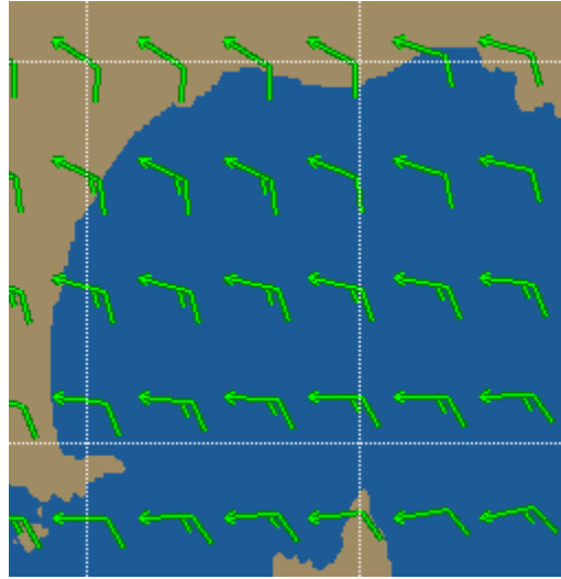
Forecast at 13.00LT (11.00UTC)
