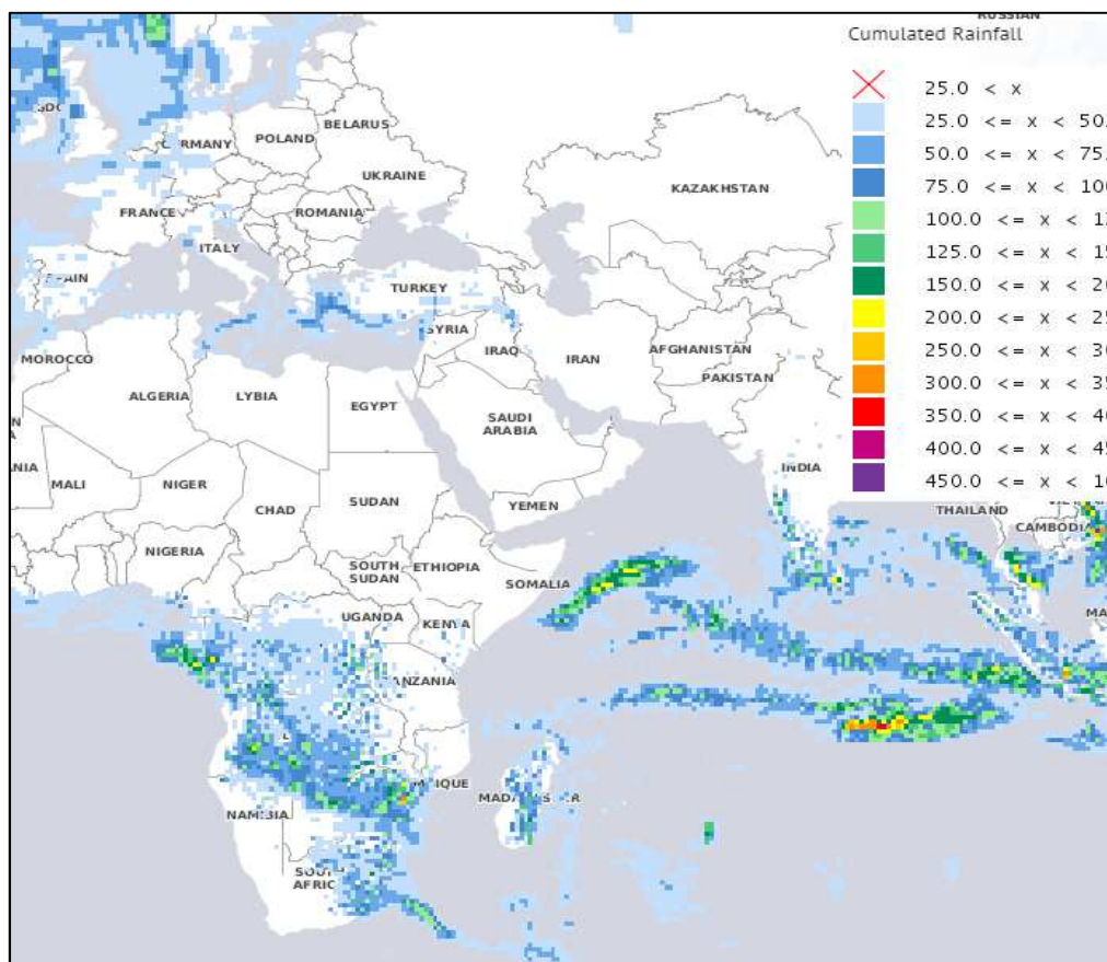
Figure 5.1 ERDS Web-GIS application, overview of 144h accumulated precipitation from GFS
