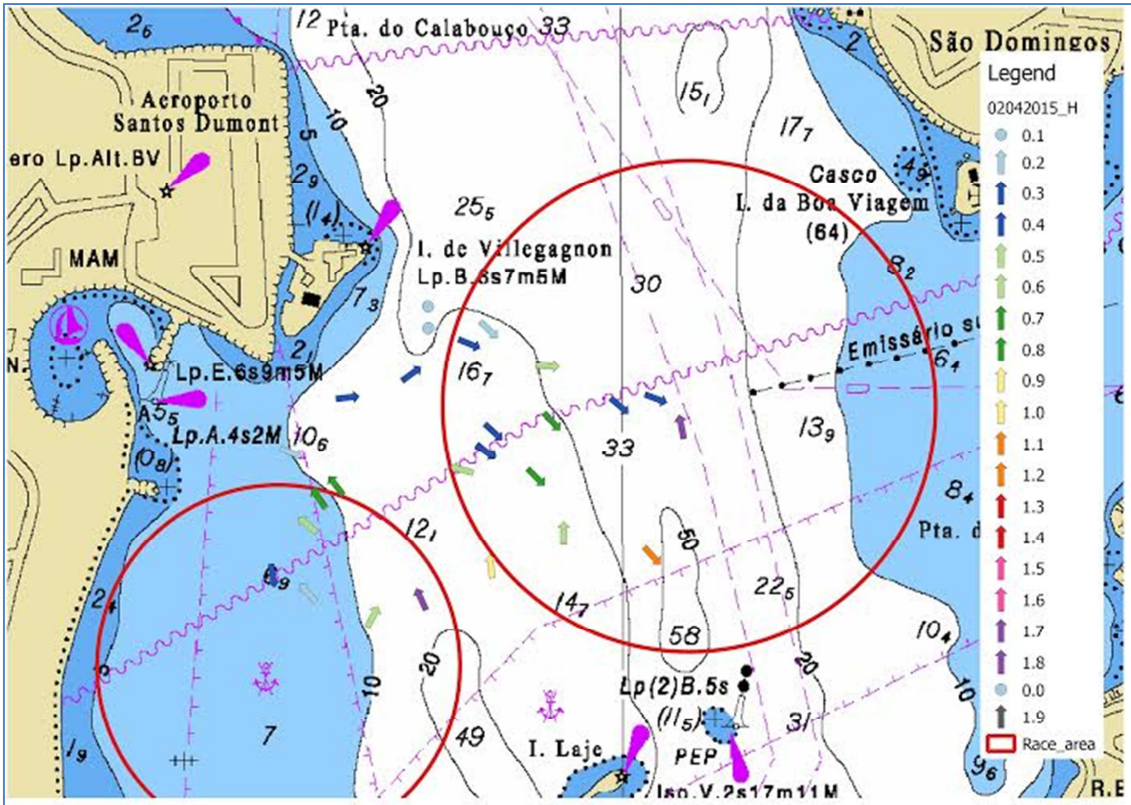
Figure 5.25 – current data visualization platform - example at High Water of 02/04/2015
