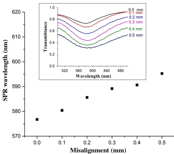
Fig. 7 The shifts of the SPR dip as a function of misalignment; inset shows the transmittance spectra.
