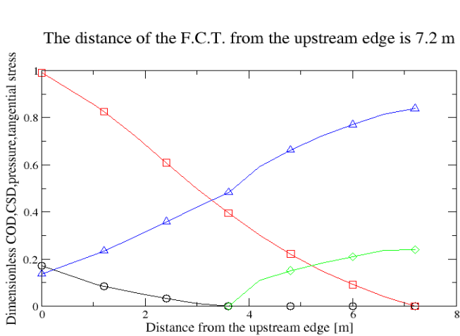
Figure 5: Results for the first step of the global stage. COD and CSD are divided by 0.8 mm. The load level is 70% of full reservoir.
