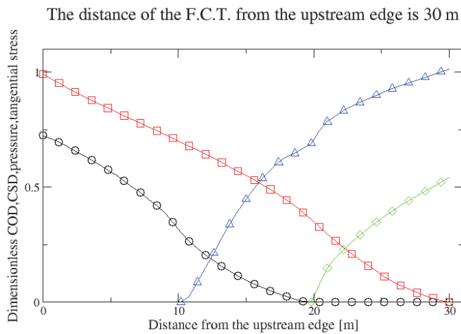
Figure 9: Results for the 5-th step of the global stage. COD and CSD are divided by 3.0 mm. The water level is 0.5 m above the dam crest.
