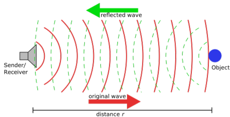
Figure 4.7: Sonar principle
