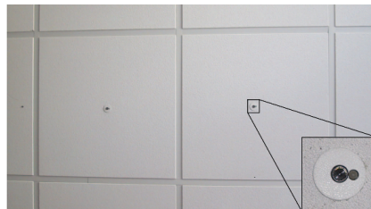
Figure 4.17: Ultrasonic receivers in ceiling tiles
