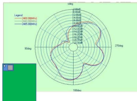
Figure 4.23: BLE 112A radio radiation pattern. Image from BLE112 documentation https://www.bluetooth.org/tpg/RefNotes/BLE112_Datasheet1.pdf .
