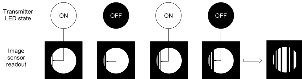
Figure 4.10: VLC data frame sample. Image from [108].
