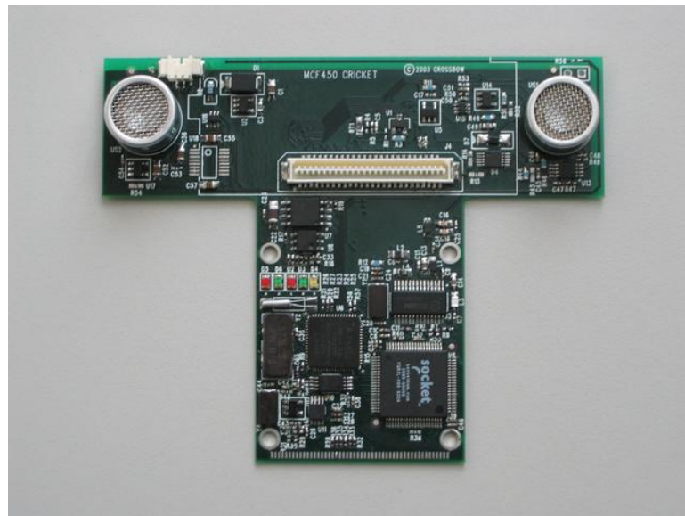
Figure 4.18: Cricket device, can act both as listener or a beacon. Image from http://cricket.csail.mit.edu/
