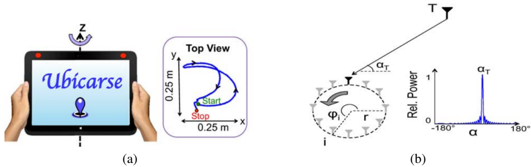
Figure 4.24: On the left is depicted the spatial movement of the mobile device. On the right it is shown how SAR is performed. Images from [80].
