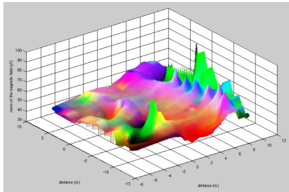
Figure 4.20: Magnetic landscape of University of Oulu Discus entrance hall. The height is the norm of the field and the color (red, green, blue) corresponds to its direction (x, y and z respectively). Image from [60].
