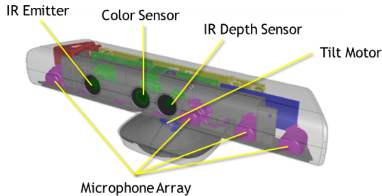
Figure 4.12: The Kinect sensor components. Picture from https://msdn.microsoft.com/en-us/library/jj131033.aspx .
