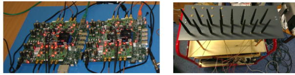
Figure 4.25: ArrayTrack access point FPGA and the antenna array. Image from [154].
