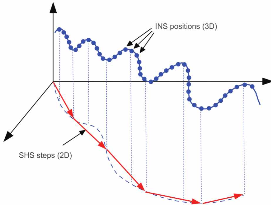
Figure 4.19: INS (Inertial Navigation system) and SHS (Step-and-heading system). An INS computes the full trajectory of a unit in 3D (solid line with position dots), whilst an SHS deals only with gross step vectors in 2D (arrow sequence). Image from [59].
