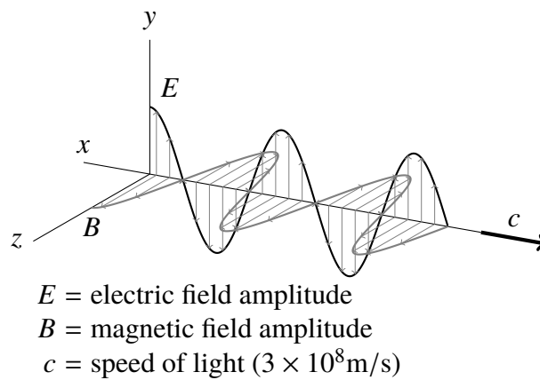
Figure 4.21: Electromagnetic wave.
