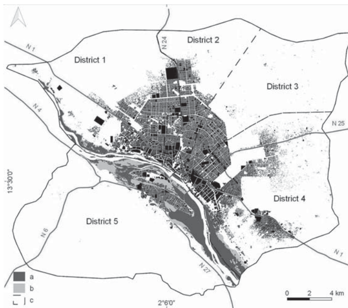
Figure 12.6: Niamey, 2014. Areas prone to river flood with (a) over 1 m water depth, (b) 0–1 m water depth, (c) districts limits, built up areas at 2014 (black) and national roads (red) (by S. Braccio)
