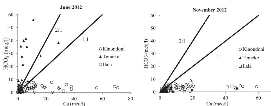
Figure 6.15: Diagram of \text{Ca}^{2+} vs. \text{HCO}_3^-
