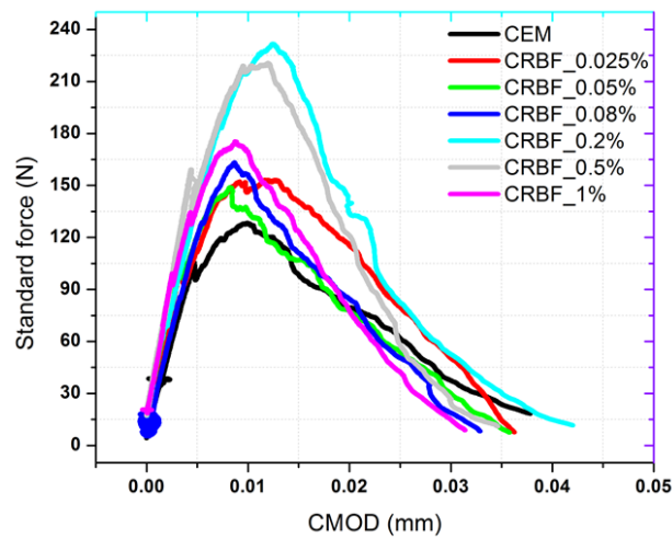
Figure 5: Typical load-CMOD curves for cement composites with and without CRBF particles additions
