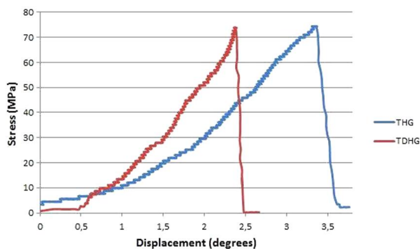
5 Typical shear stress–displacement curve obtained for torsion test of THG and TDHG hourglass joined samples
